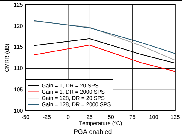
Figure 23. DC CMRR vs Temperature
