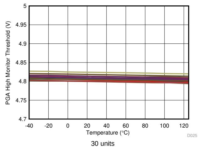
Figure 36. PGA High Monitor Threshold vs Temperature
