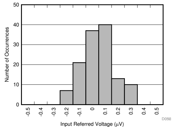
Gain = 128, 10 SPS, after offset calibration, 128 samples Figure 7-55. ADC2 Output Reading Distribution
