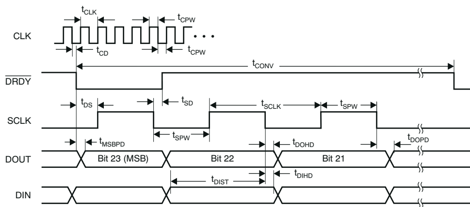
Figure 5-1. SPI Format Timing Characteristics
