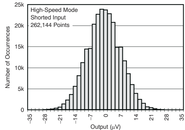
Figure 5-6. Noise Histogram
