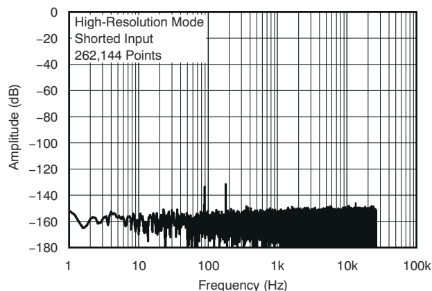
Figure 5-9. Output Spectrum
