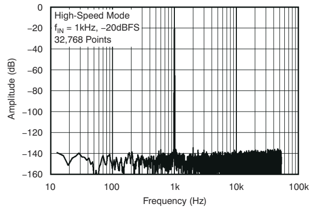
Figure 5-4. Output Spectrum
