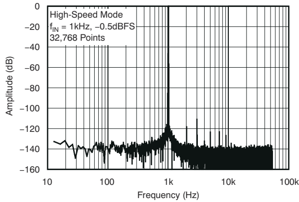
Figure 5-3. Output Spectrum
