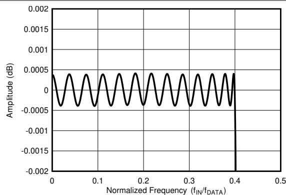
Figure 7-14. Wideband Filter Pass-Band Ripple
