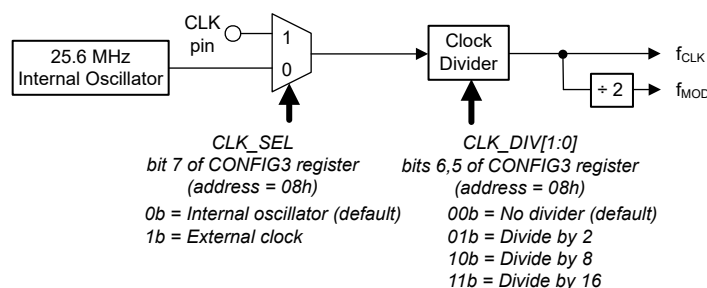
Figure 7-6. Clock Block Diagram
