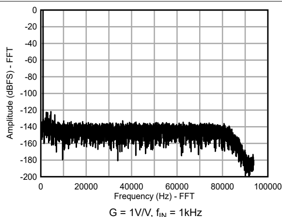
Figure 9-5. Wideband Filter Performance
