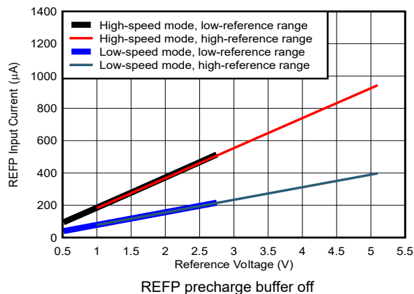
Figure 5-77. REFP Input Current vs Reference Voltage
