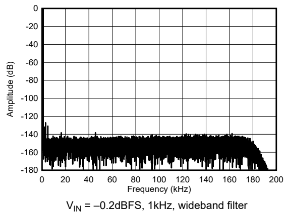
Figure 5-18. High-Speed Mode, Full-Scale FFT
