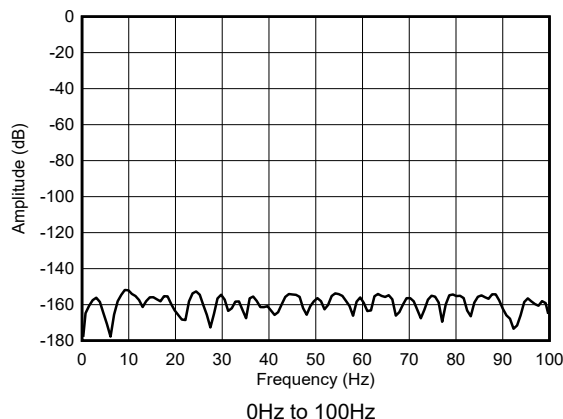
Figure 5-14. High-Speed Mode, Shorted-Input FFT
