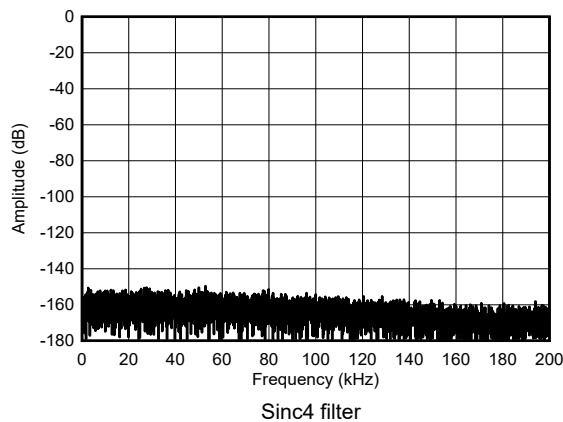
Figure 5-16. High-Speed Mode, Shorted-Input FFT
