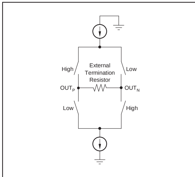
Figure 18. LVDS Buffer
