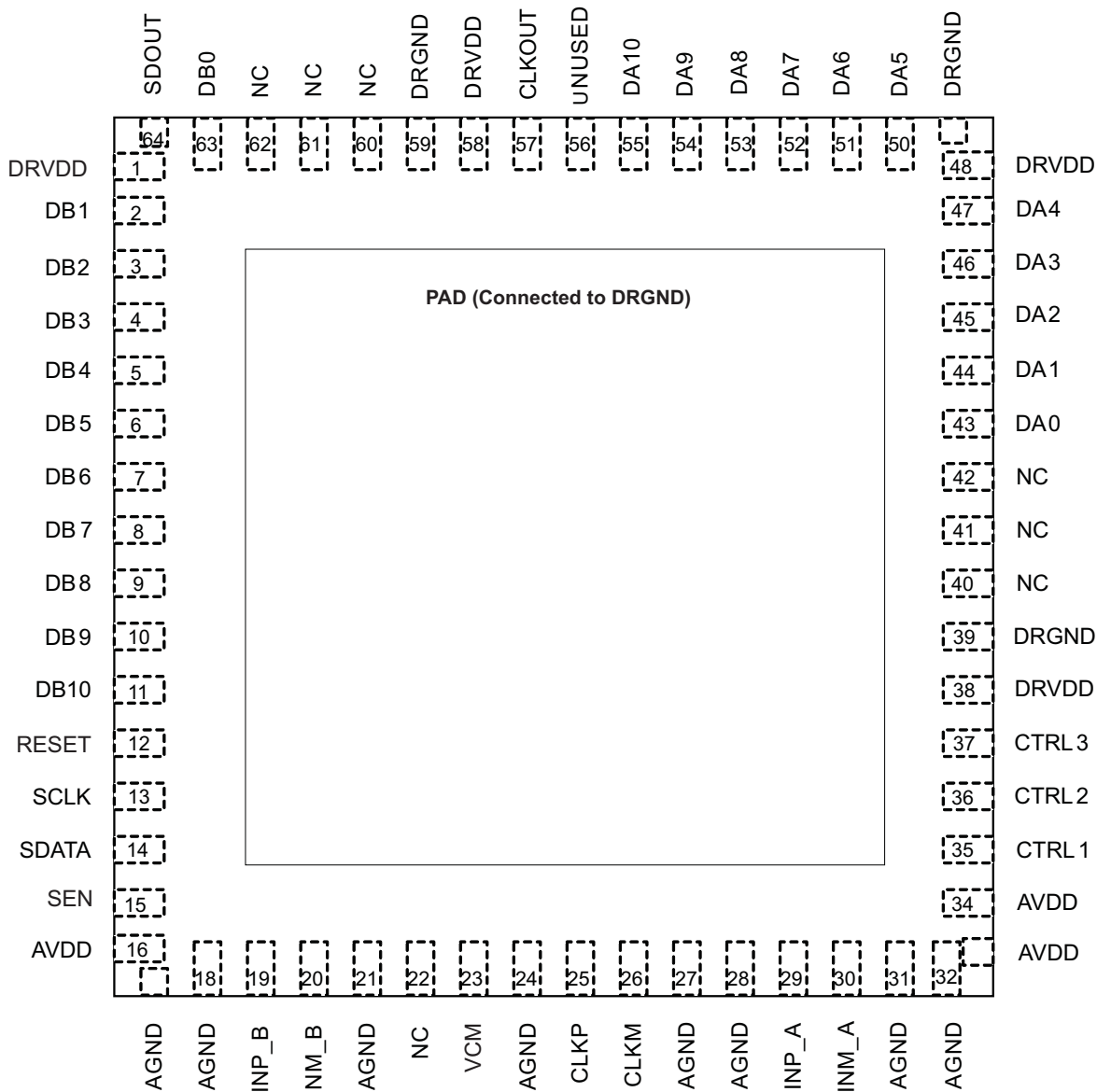
Figure 11. Pin Configuration
