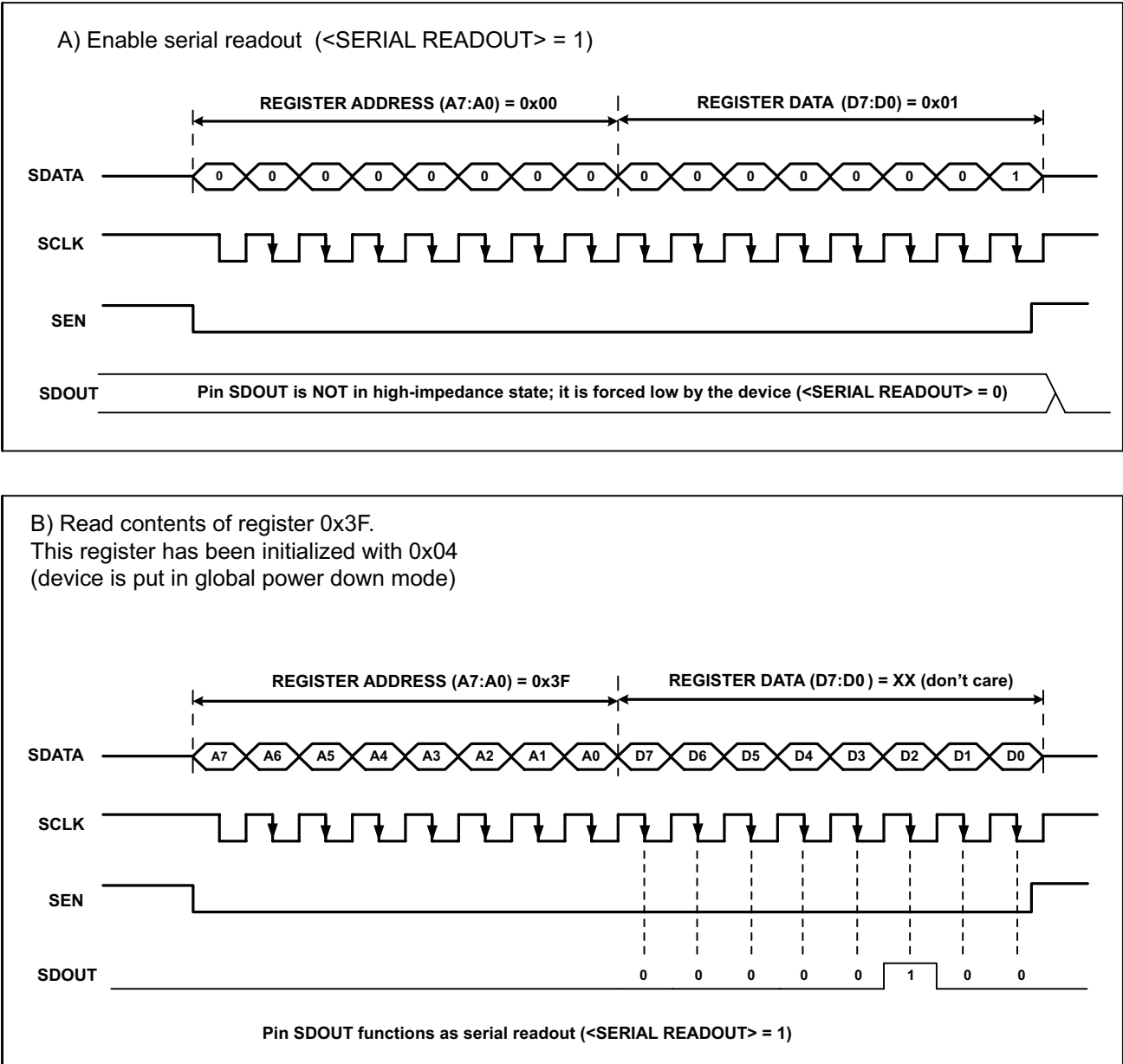
Figure 8. Serial Readout
