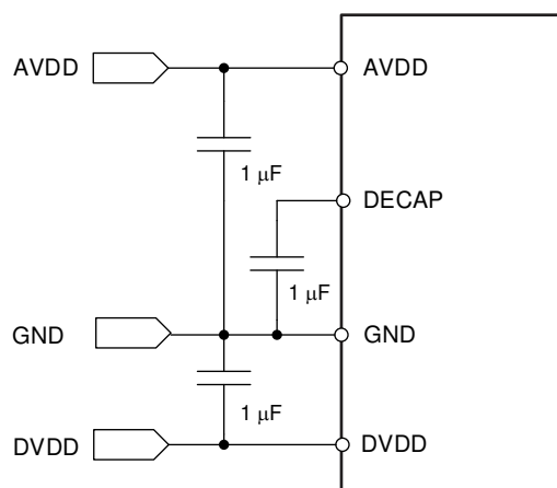
Figure 161. Power-Supply Decoupling
