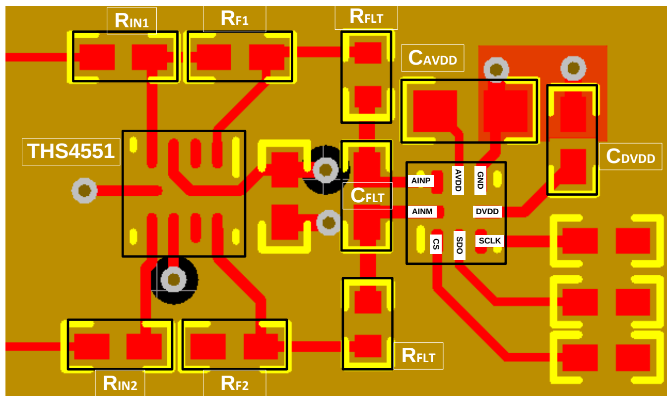
Figure 48. Example Layout
