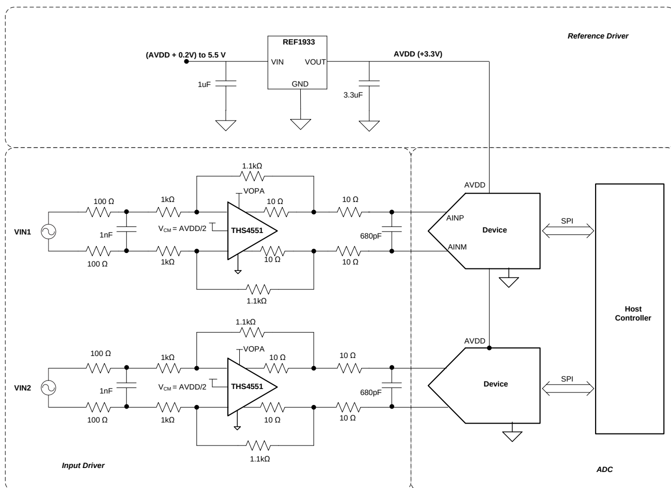
Figure 40. 2-Channel, Simultaneous-Sampling Data Acquisition (DAQ) Circuit Using the ADS7054
