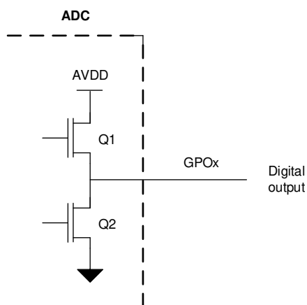
Figure 159. Digital Push-Pull Output
