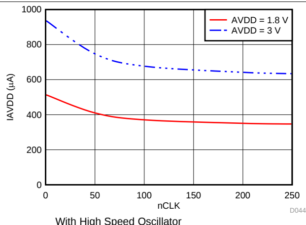
Figure 74. I_{AVDD} in High Precision Mode with nCLK
