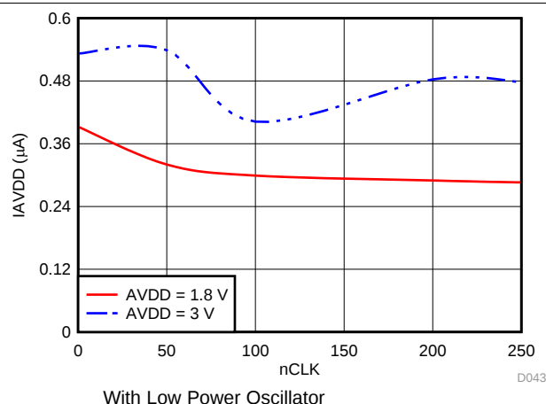
Figure 73. I_{AVDD} in High Precision Mode with nCLK
