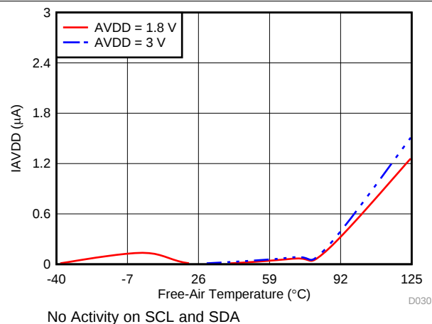
Figure 28. Static I_{AVDD} in Manual Mode with Temperature
