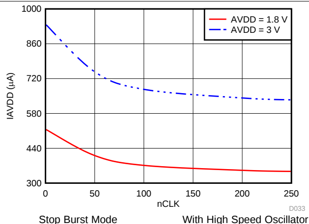
Figure 72. I_{AVDD} in Autonomous Modes with nCLK
