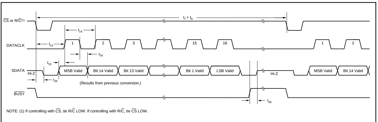
FIGURE 4. Serial Data Timing Using Internal Data Clock ( \overline{TAG} LOW).
