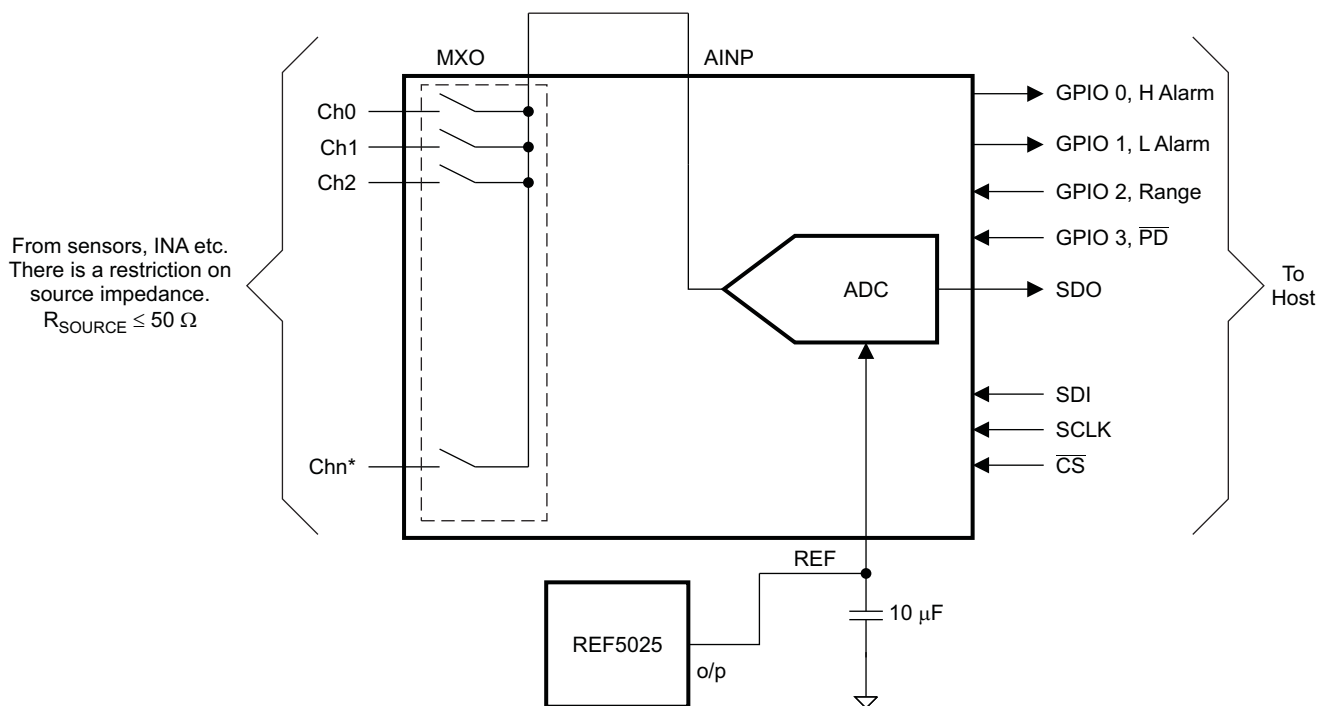
Figure 17. Typical Application Diagram Showing MXO Shorted to AINP
