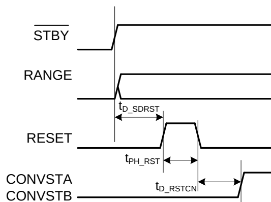
Figure 9. Exit Shutdown Mode Timing Diagram
