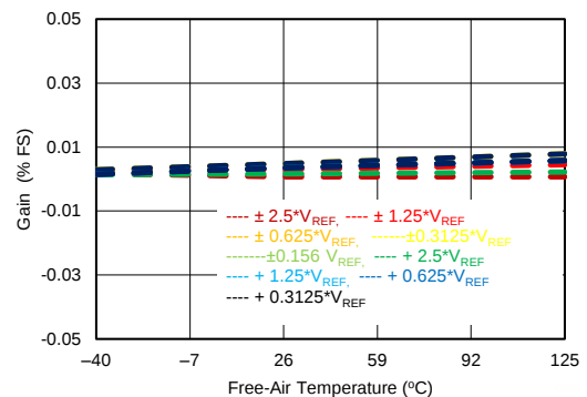
Gain Error versus Temperature
