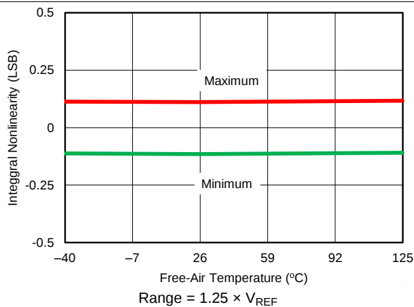
Figure 30. INL vs Temperature ( 1.25 \times V_{REF} )
