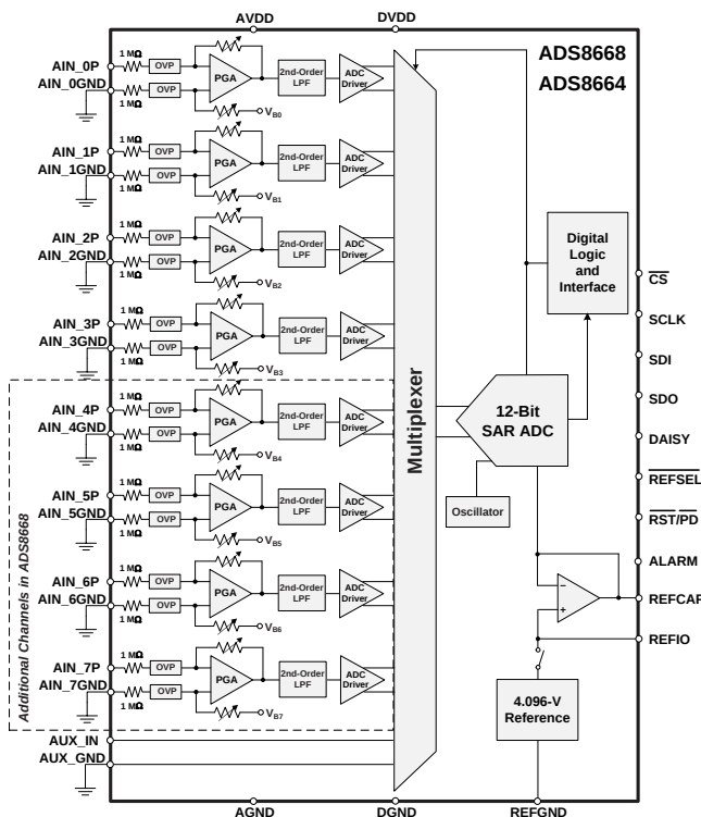
Block Diagram
