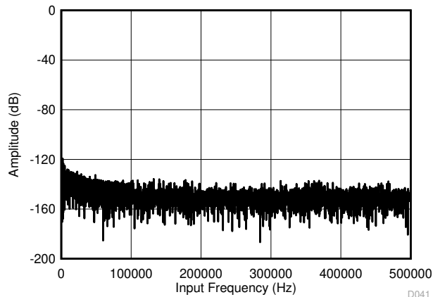
Figure 6-33. Typical FFT Plot (All Ranges) for the ADS8681
