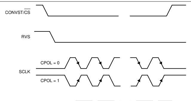
Figure 7-33. Standard SPI Timing Protocol (CPHA = 1, Single SDO-x)
