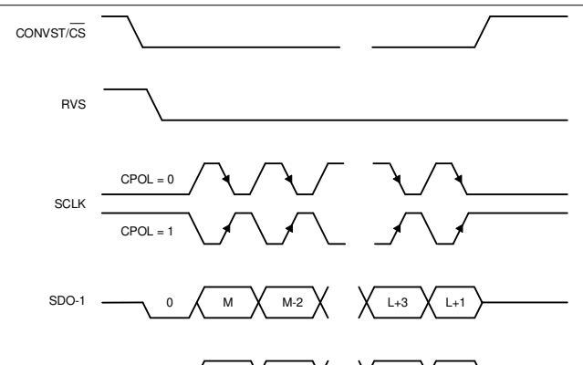
Figure 7-35. Standard SPI Timing Protocol (CPHA = 1, Dual SDO-x)
