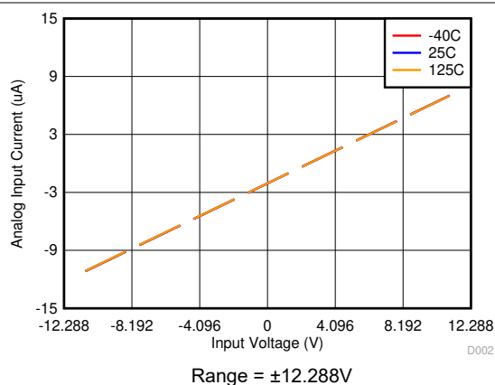
Figure 5-10. Input I-V Characteristic Across Temperature
