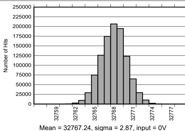
Figure 5-14. DC Histogram for Midscale Inputs (±10.24V)
