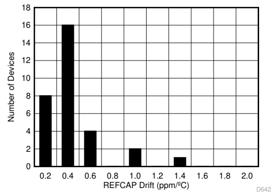
Figure 6-14. Reference Buffer Temperature Drift Histogram
