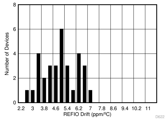
Figure 6-11. Internal Reference Temperature Drift Histogram
