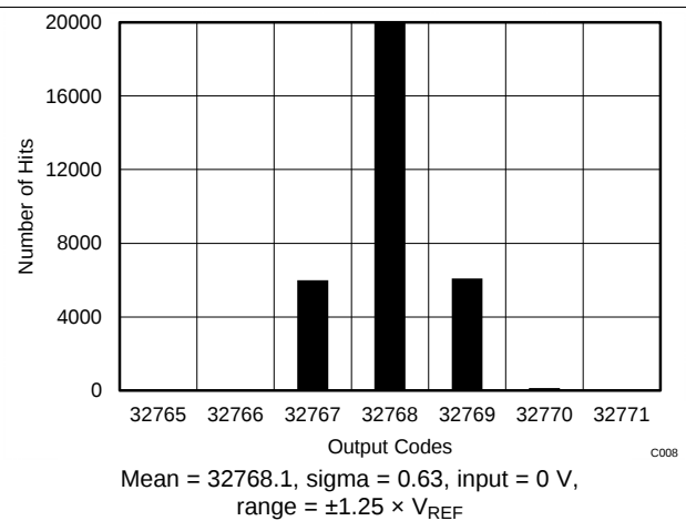
Figure 7. DC Histogram for Mid-Scale Inputs ( \pm 1.25 \times V_{REF} )
