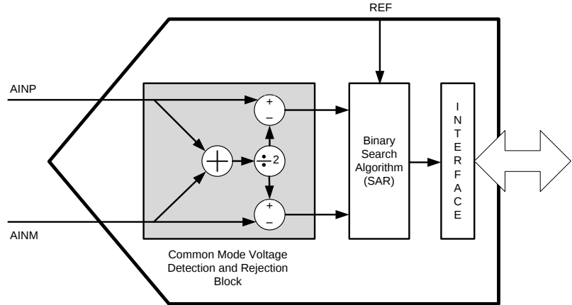
Figure 46. Conceptual Diagram: True Differential Input Structure
