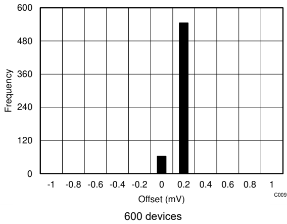
Figure 5-25. Offset Typical Distribution
