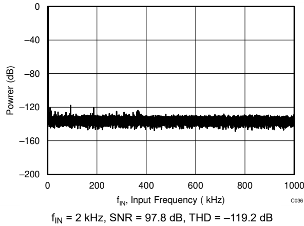
Figure 7-9. FFT with a 2-kHz Input Signal, Single-Ended Input
