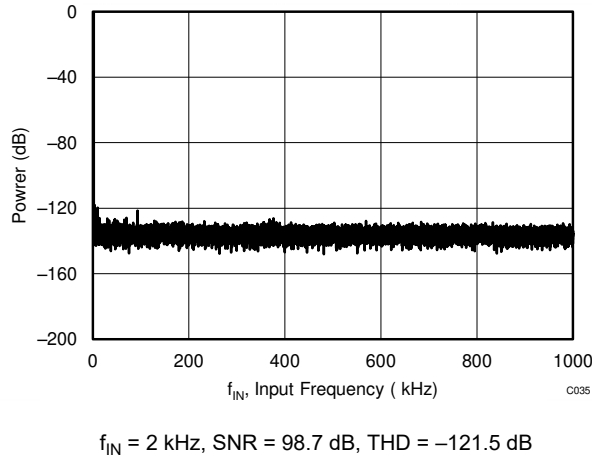
Figure 7-7. FFT with a 2-kHz Input Signal, Differential Input
