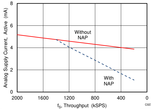
Figure 8-4. Power Scaling with Throughput with NAP Mode
