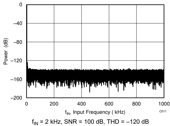
Figure 5-17. Typical FFT
