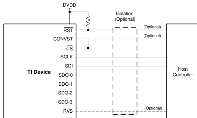
Figure 6-47. SPI Interface, Minimum Pins
