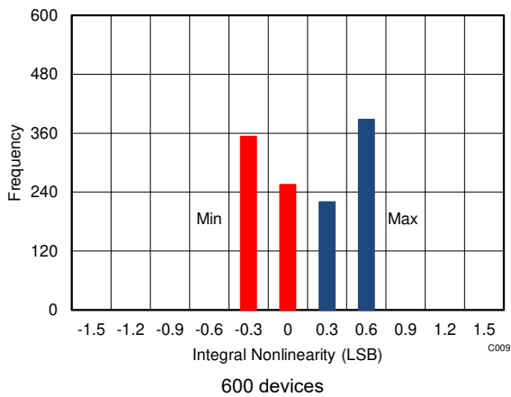
Figure 5-9. Typical INL Distribution
