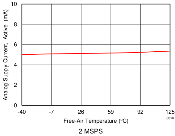
Figure 5-31. Supply Current vs Temperature
