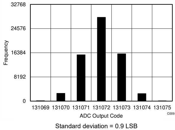
Figure 5-15. DC Input Histogram, Code Center
