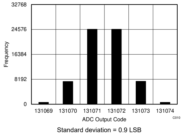
Figure 5-16. DC Input Histogram, Code Transition
