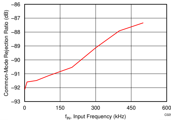
Figure 5-35. CMRR vs Input Frequency
