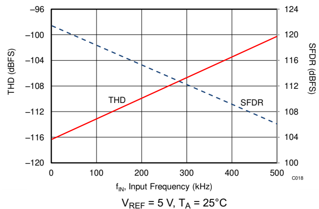
Figure 5-24. Distortion Performance vs Input Frequency
