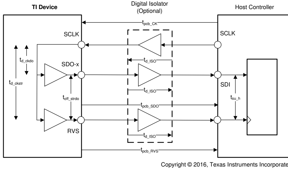
Figure 6-16. Delays in Source-Synchronous Communication
