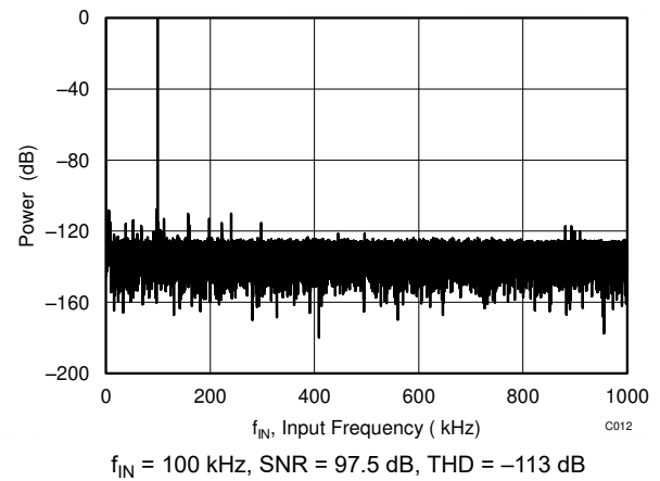
Figure 5-18. Typical FFT
