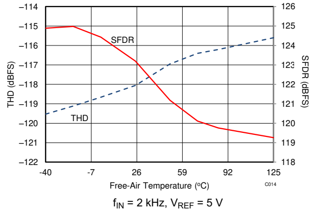
Figure 5-20. Distortion Performance vs Temperature
