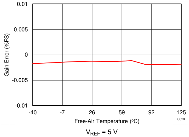
Figure 5-28. Gain Error vs Temperature
