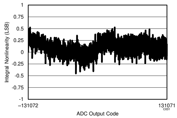
Figure 7-4. Typical INL
