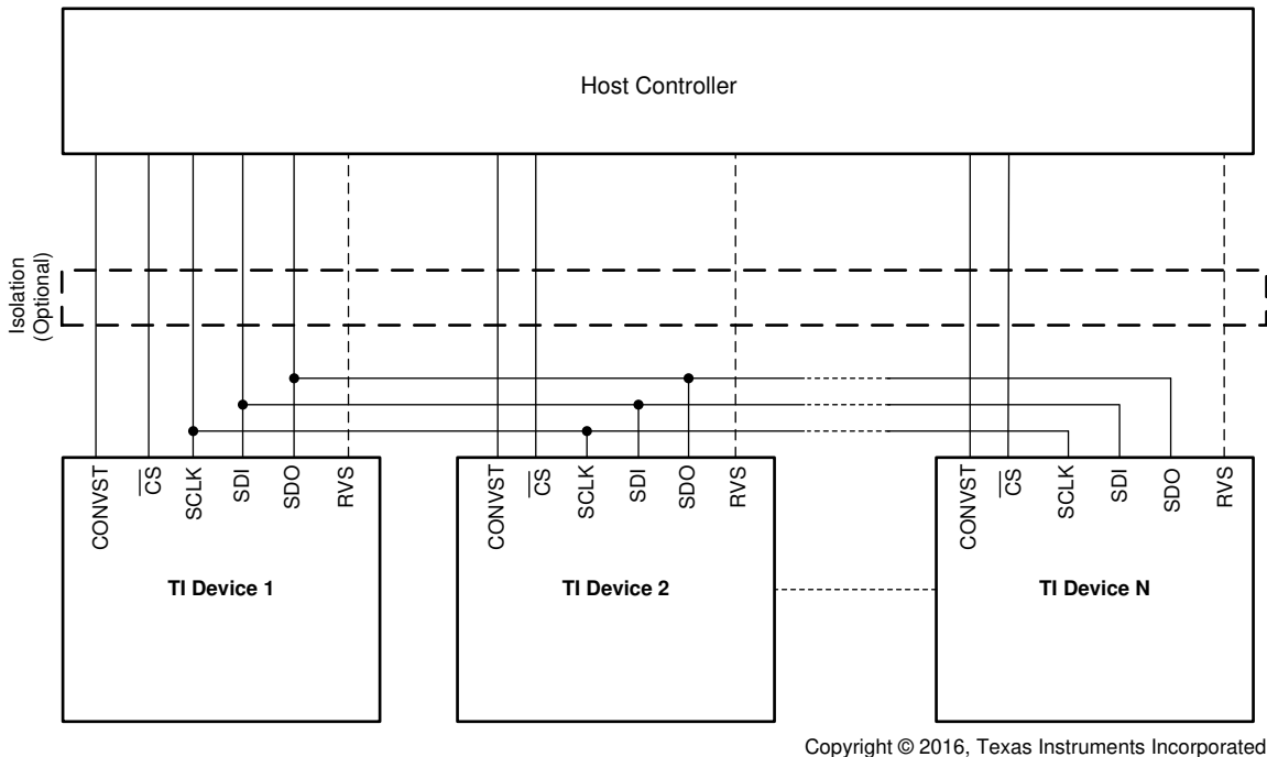
Figure 6-51. Star Topology Connection
