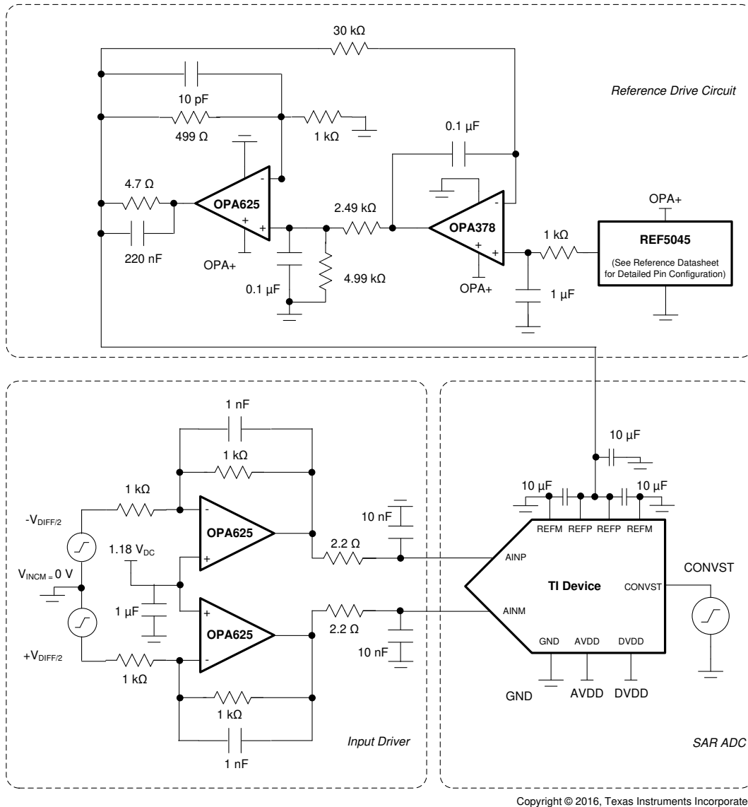
Figure 7-2. Differential Input DAQ Circuit for Lowest Distortion and Noise at 2 MSPS
