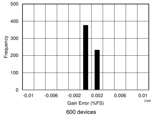
Figure 5-26. Gain Error Typical Distribution
