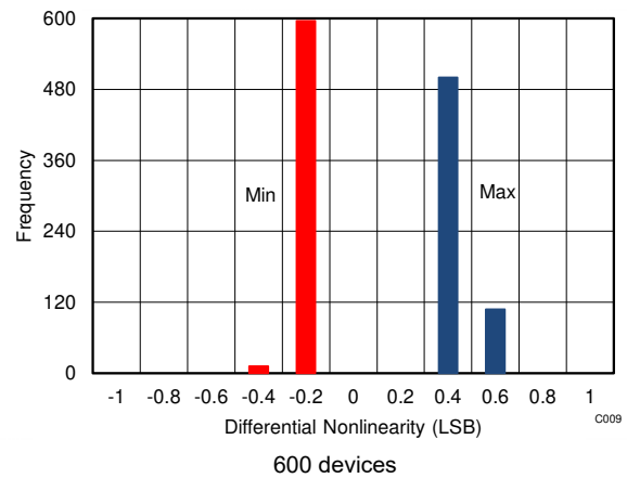
Figure 5-10. Typical DNL Distribution
