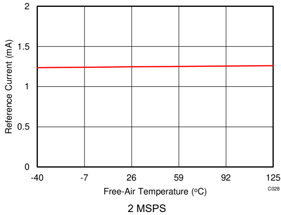
Figure 5-33. Reference Current vs Temperature
