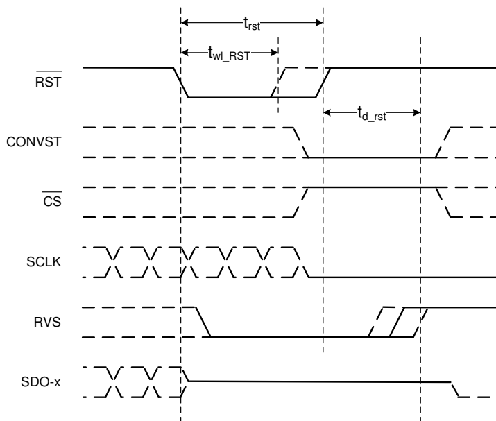
Figure 6-7. Asynchronous Reset
