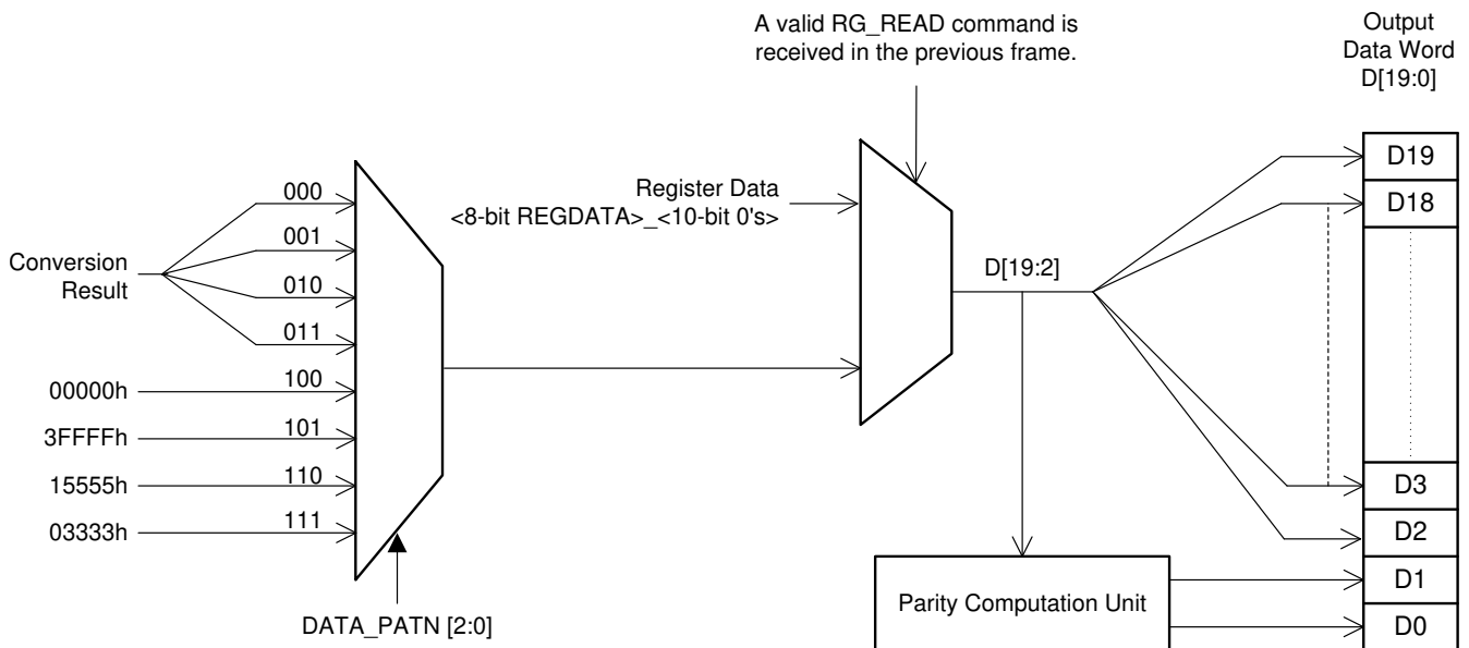
Figure 6-9. Output Data Word (D[19:0])
