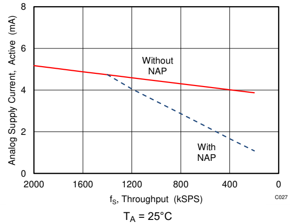
Figure 5-32. Supply Current vs Throughput
