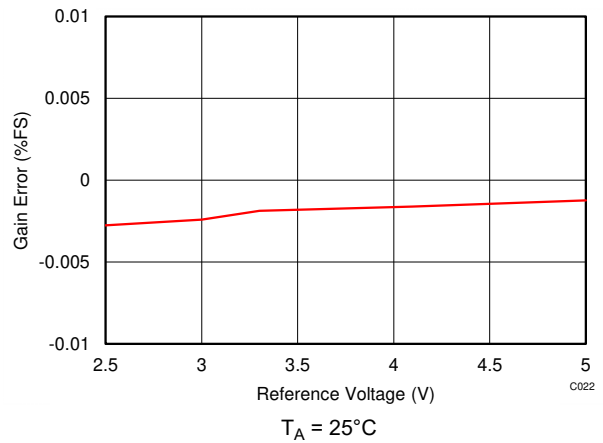
Figure 5-30. Gain Error vs Reference Voltage
