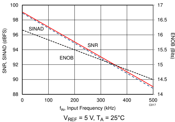
Figure 5-23. Noise Performance vs Input Frequency
