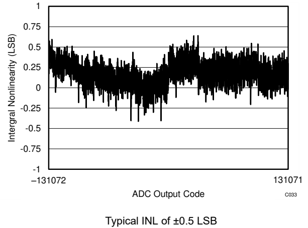
Figure 7-10. Typical INL, Single-Ended Input
