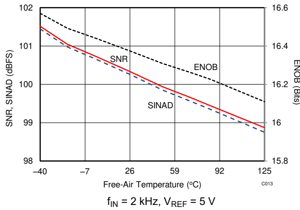
Figure 5-19. Noise Performance vs Temperature
