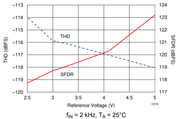
Figure 5-22. Distortion Performance vs Reference Voltage
