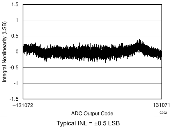
Figure 5-7. Typical INL
