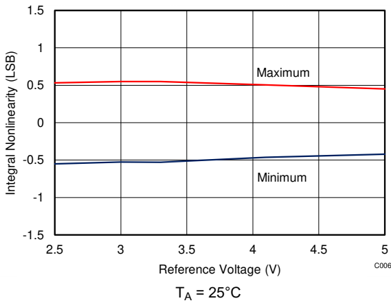
Figure 5-13. INL vs Reference Voltage
