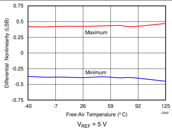
Figure 5-12. DNL vs Temperature
