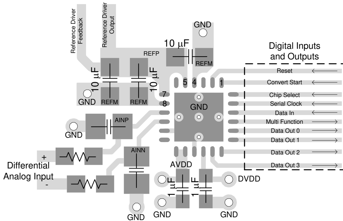
Figure 9-1. Recommended Layout
