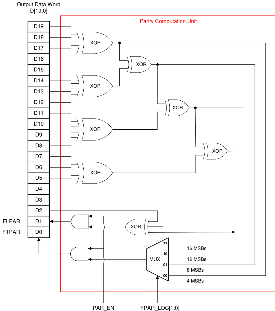
Figure 6-10. Parity Bits Computation
