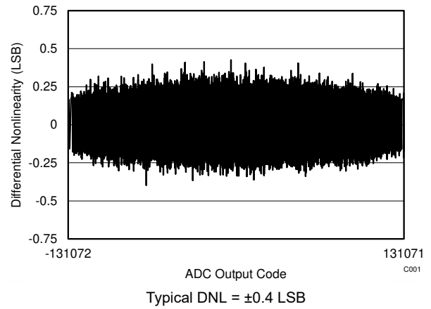
Figure 5-8. Typical DNL
