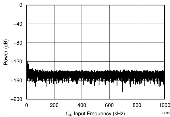
Figure 7-3. FFT with a 2-kHz Input Signal
