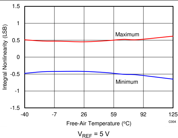
Figure 5-11. INL vs Temperature
