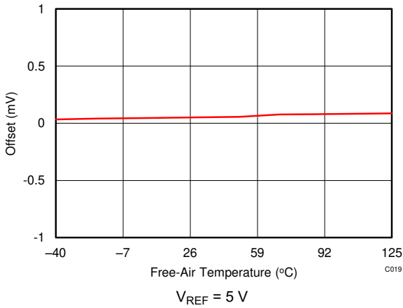
Figure 5-27. Offset vs Temperature
