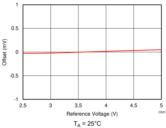
Figure 5-29. Offset vs Reference Voltage
