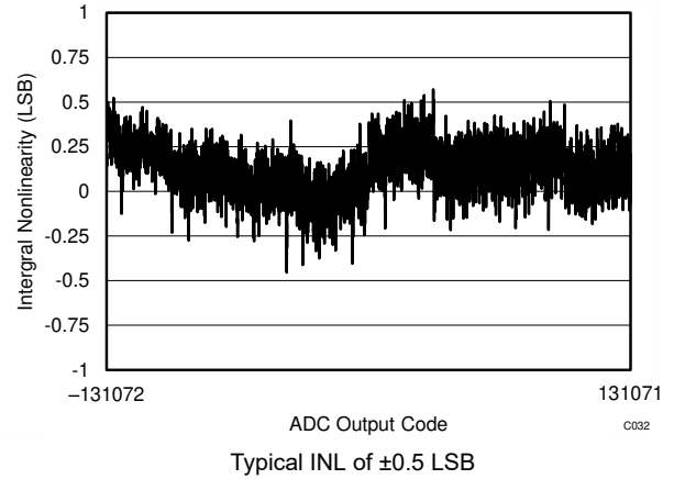
Figure 7-8. Typical INL, Differential Input
