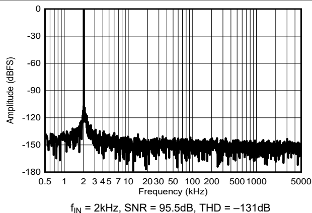
Figure 6-24. Typical FFT for f_{IN} = 2\text{kHz}
