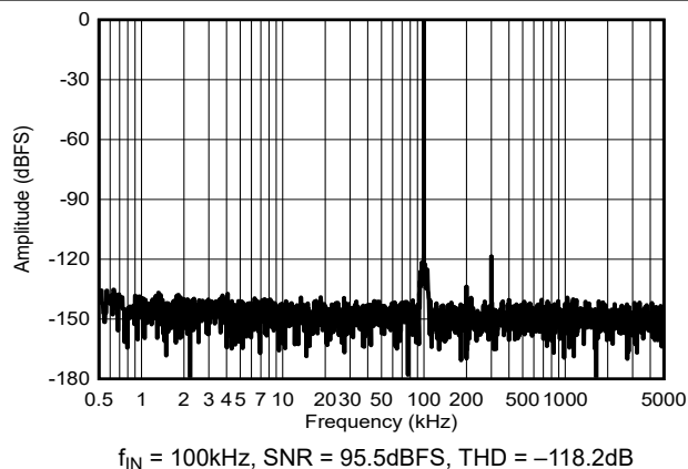
Figure 6-25. Typical FFT for f_{IN} = 100\text{kHz}
