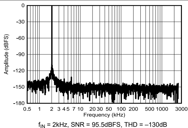
Figure 9-2. Typical FFT at 5MSPS/Channel: ADS9117
