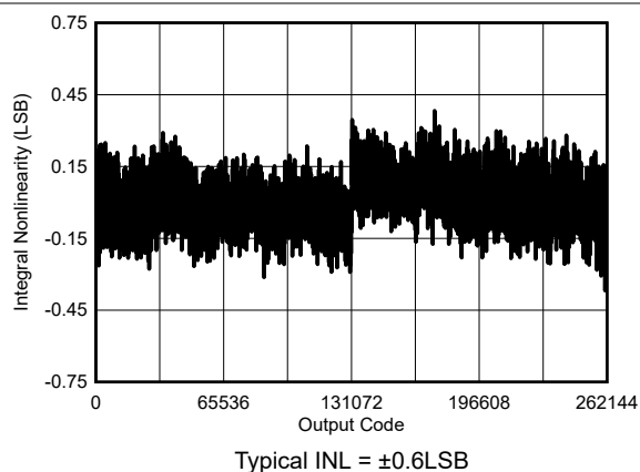
Figure 6-22. Typical INL
