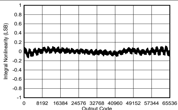
Figure 5-17. Typical INL
