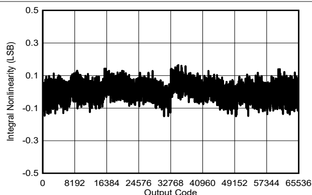
Typical INL = \pm 0.2\text{LSB} Figure 5-27. Typical INL
