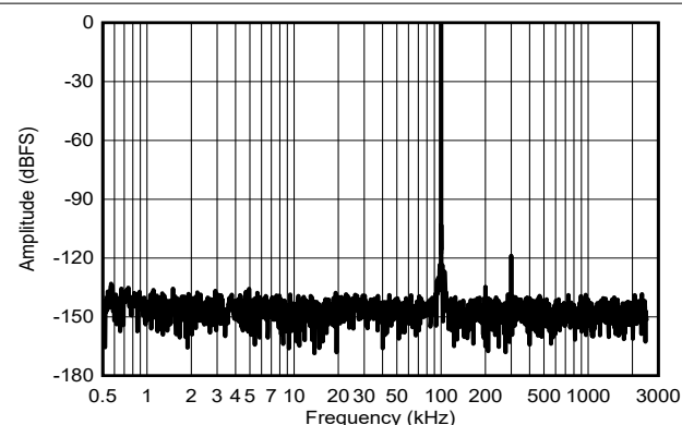
f_{IN} = 100\text{kHz} , SNR = 93.8dBFS, THD = -119dB Figure 5-30. Typical FFT for f_{IN} = 100\text{kHz}
