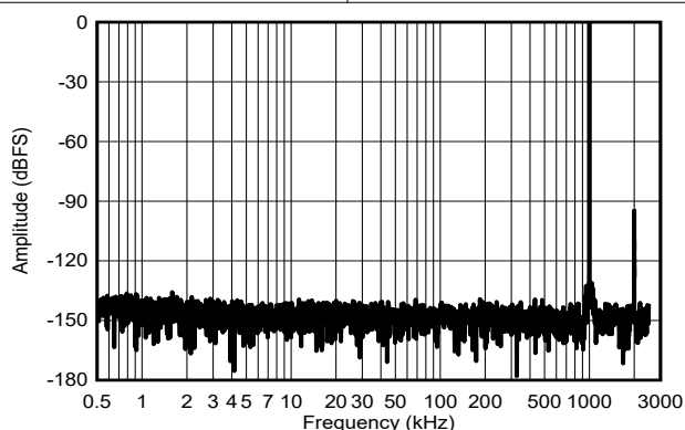
f_{IN} = 1\text{MHz} , SNR = 93.3dBFS, THD = -104.5dB Figure 5-31. Typical FFT for f_{IN} = 1\text{MHz}
