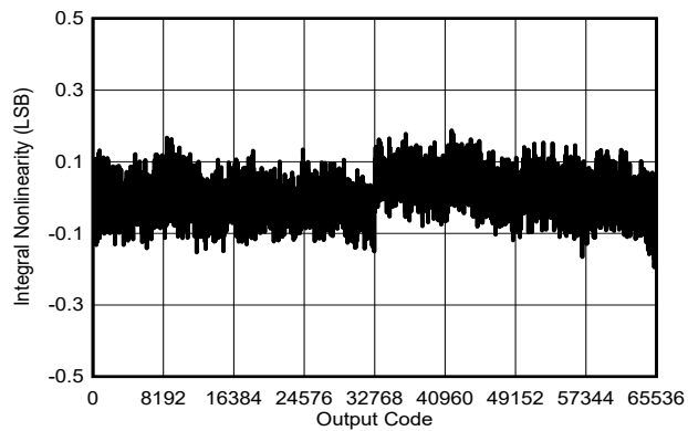
Figure 5-22. Typical INL
