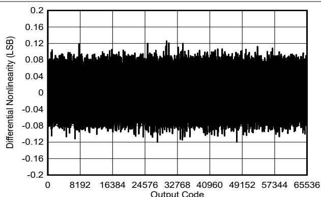
Typical DNL = \pm 0.15\text{LSB} Figure 5-28. Typical DNL
