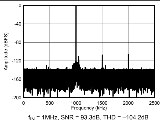
Figure 8-9. Typical FFT at 5MSPS: ADS9127
