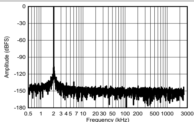
f_{IN} = 2\text{kHz} , SNR = 93.9dBFS, THD = -122.5dB Figure 5-29. Typical FFT for f_{IN} = 2\text{kHz}
