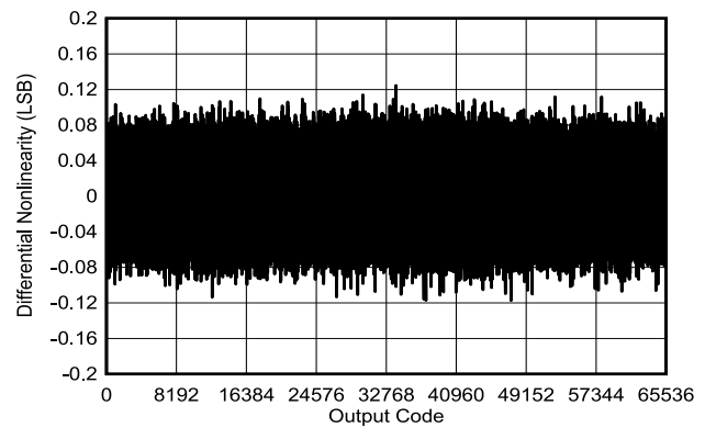
Figure 5-23. Typical DNL
