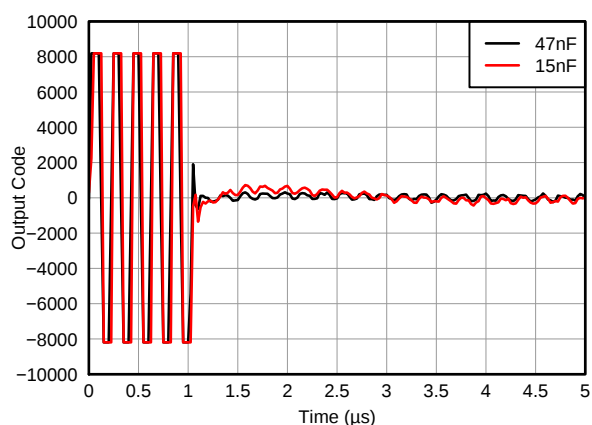
Figure 53. Overload Recovery Response vs. INM Capacitor, V_{IN} = 50 \text{ mV}_{PP}/100 \text{ } \mu\text{V}_{PP} , Max Gain
