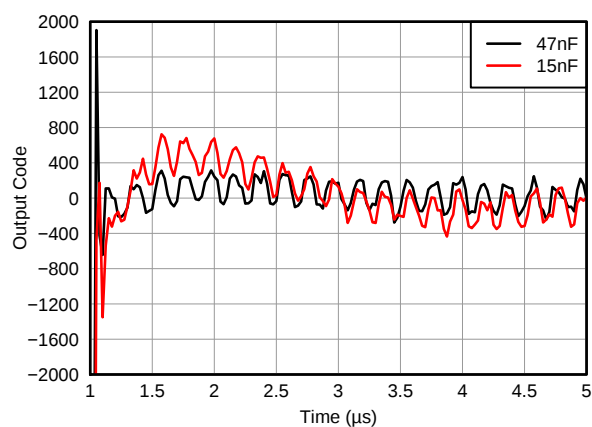
Figure 54. Overload Recovery Response vs. INM Capacitor (Zoomed), V_{IN} = 50 \text{ mV}_{PP}/100 \text{ } \mu\text{V}_{PP} , Max Gain
