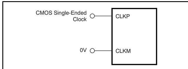
Figure 105. Single-Ended Clock Driving Circuit (DIFF_CLK = 0)
