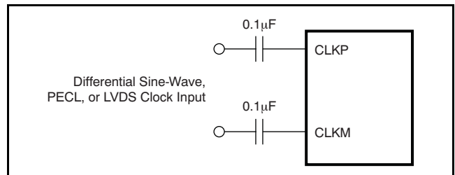
Figure 107. Differential Clock Driving Circuit (DIFF_CLK = 1)
