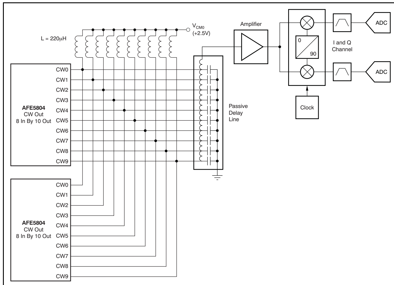
Figure 104. Conceptual CW Doppler Signal Path Using Current Summing and a Passive Delay Line for Beam-Forming
