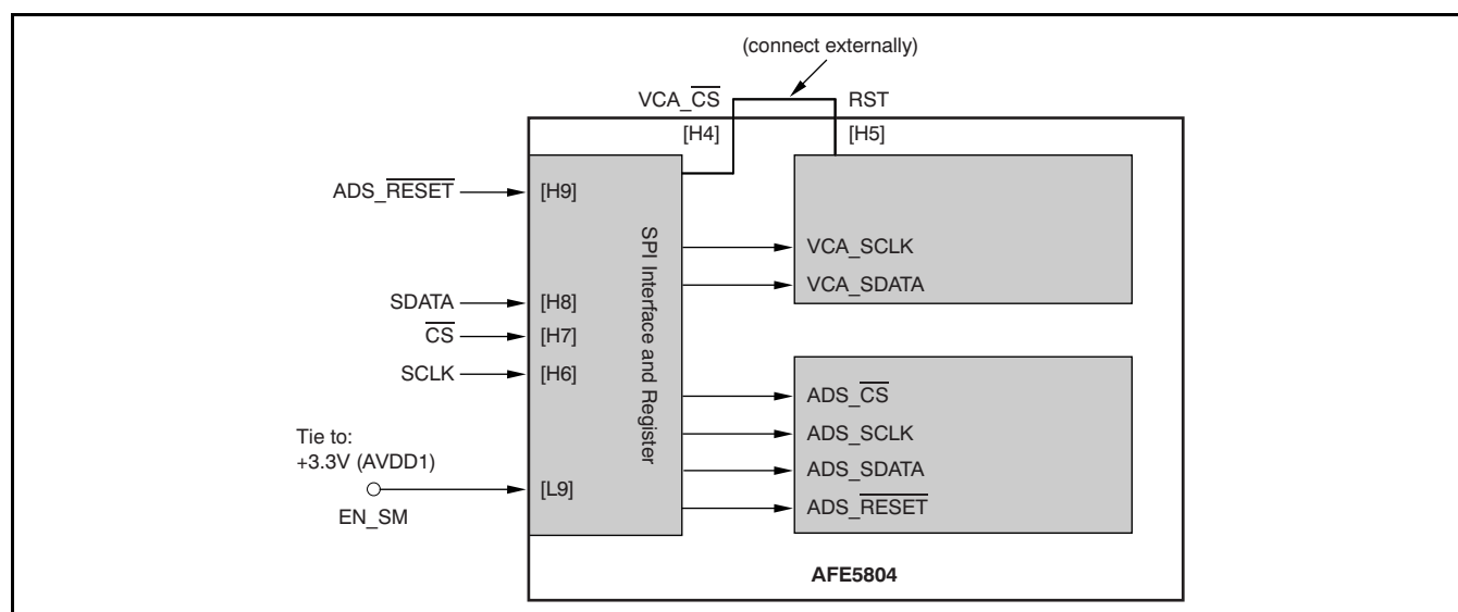
Figure 92. Typical Connection Diagram for the SPI Control Lines
