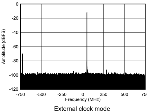
Figure 4-442. RX Single Tone Output FFT at 8.11GHz, -12dBFS
