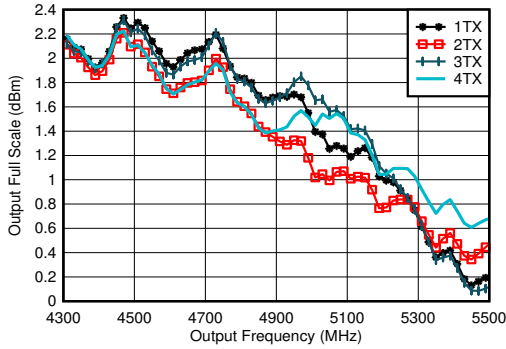
Excluding PCB and cable losses, A_{\text{out}} = -0.5\text{ dBFS} , DSA = 0, 4.9GHz matching
