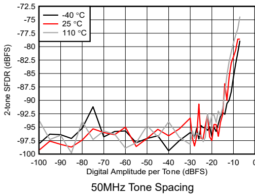
Figure 4-440. RX 2-tone SFDR vs Digital Amplitude at 8.11GHz
