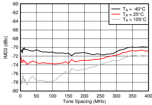
f_{\text{DAC}} = 8847.36\text{MSPS} , straight mode, f_{\text{CENTER}} = 2.6\text{GHz} , matching at 2.6GHz, -13\text{ dBFS} each tone, worst channel.
