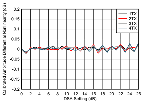
Figure 4-237. TX DSA Calibrated Amplitude Differential Nonlinearity
