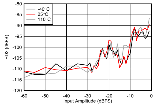
Figure 4-462. RX HD2 vs Digital Level at 9.6GHz
