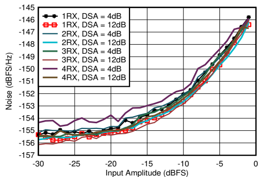
Figure 4-407. RX Noise Spectral Density vs Input Amplitude and Channel at 4.9GHz
