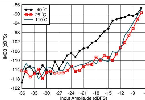
Figure 5-295. RX IMD3 vs Input Level and Temperature at 0.8 GHz
