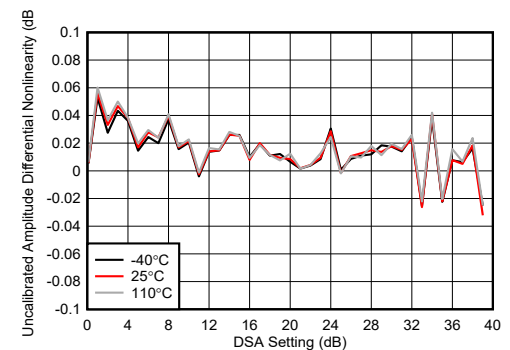
Figure 5-189. TX DSA Uncalibrated Amplitude Differential Nonlinearity at 8.11 GHz
