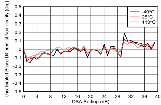
Figure 5-197. TX DSA Uncalibrated Phase Differential Nonlinearity at 8.11 GHz
