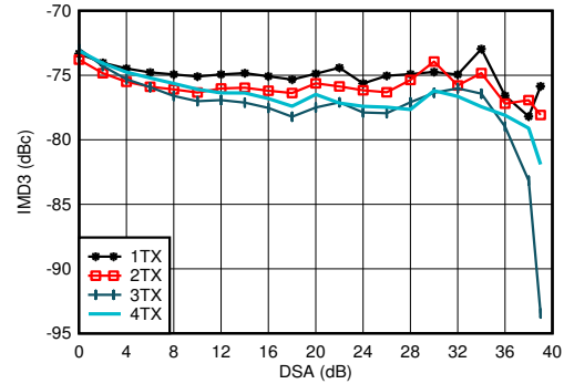
Figure 5-97. TX IMD3 vs DSA Setting at 2.6 GHz
