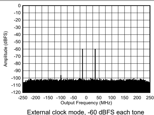
Figure 5-443. RX Dual Tone Output FFT at 8.1 GHz
