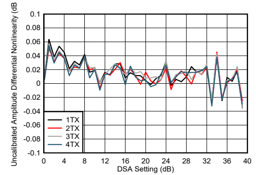
Figure 5-187. TX DSA Uncalibrated Amplitude Differential Nonlinearity at 8.11 GHz
