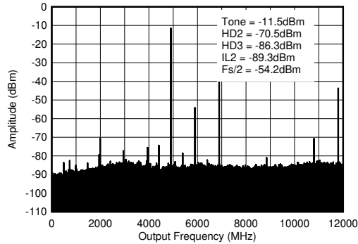
Figure 5-181. TX Single Tone (-12 dBFS) Output Spectrum at 4.9 GHz ( 0-f_{\text{DAC}} )
