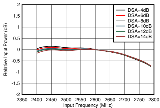
Figure 5-339. RX Inband Gain Flatness, f_{\text{IN}} = 2600\text{ MHz}
