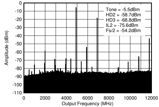
Figure 5-182. TX Single Tone (-6 dBFS) Output Spectrum at 4.9 GHz ( 0-f_{\text{DAC}} )
