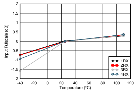
Figure 5-340. RX Input Fullscale vs Temperature and Channel at 2.6 GHz
