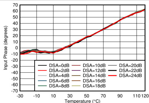
Figure 5-360. RX Input Phase vs Temperature at 3.6 GHz
