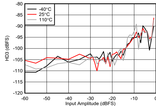
Figure 4-437. RX HD3 vs Digital Amplitude at 8.1GHz
