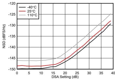
Figure 4-263. TX NSD vs DSA Setting at 9.61 GHz
