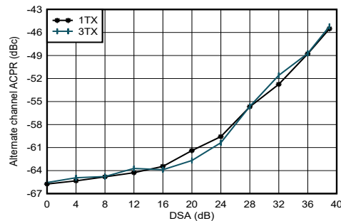
Figure 4-227. TX NR100 MHz alt-ACPR vs DSA Setting 8.1 GHz
