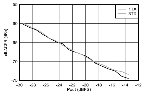
Figure 4-105. TX 20-MHz LTE alt-ACPR vs Digital Level at 2.6 GHz
