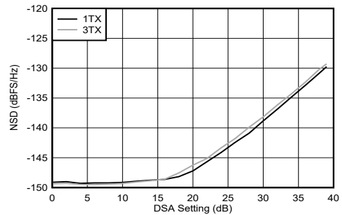
Figure 4-262. TX NSD vs DSA Setting at 9.61 GHz
