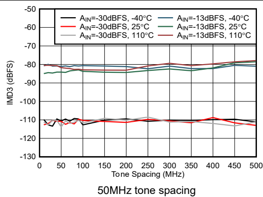
Figure 4-457. RX IMD3 vs Tone Spacing at 9.6 GHz
