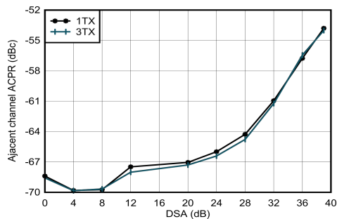
Figure 4-35. TX 20-MHz LTE ACPR vs DSA at 0.85 GHz
