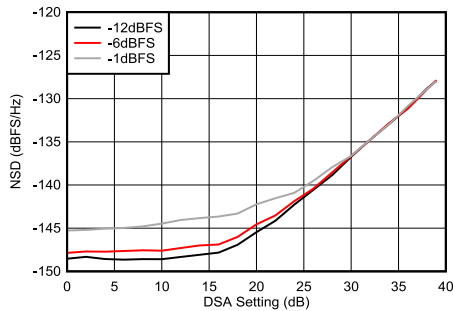
Figure 4-261. TX NSD vs DSA Setting at 9.61 GHz
