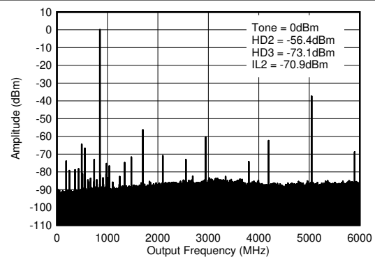
f_{\text{DAC}} = 5898.24 MSPS, interleave mode, 0.8 GHz matching, includes PCB and cable losses. \text{ILn} = f_{\text{S}}/n \pm f_{\text{OUT}} .
