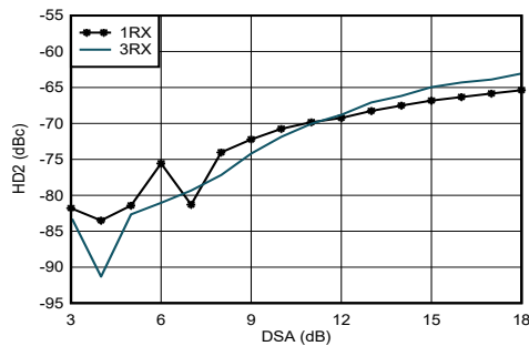
Figure 4-305. RX HD2 vs DSA Setting and Channel at 0.8 GHz
