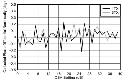
Figure 4-196. TX DSA Calibrated Phase Differential Nonlinearity at 8.11 GHz
