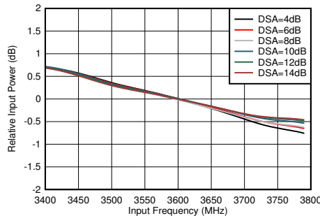
Figure 4-366. RX In-Band Gain Flatness, f_{\text{IN}} = 3600 \text{ MHz}
