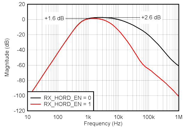
Figure 6-52. HART Internal Mode Complete Band-Pass Filter Response (From HART_RX Signal to Internal Demodulator)
