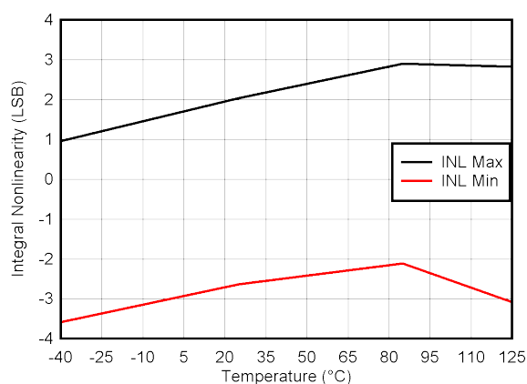
Figure 6-38. ADC INL Range vs Temperature
