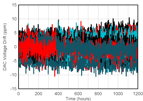
Figure 6-33. DAC Output Voltage Long-Term Stability
