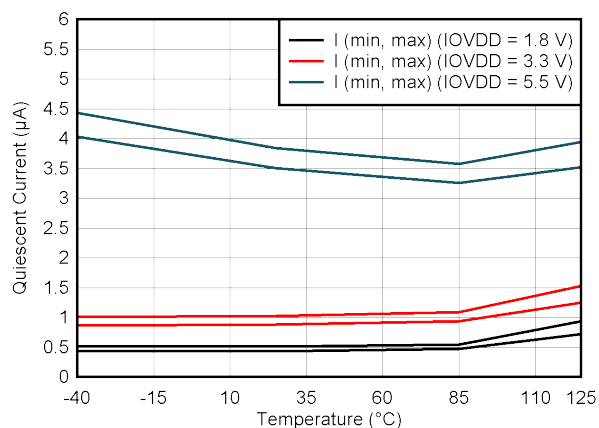
Figure 6-54. IOVDD Supply Current vs Temperature
