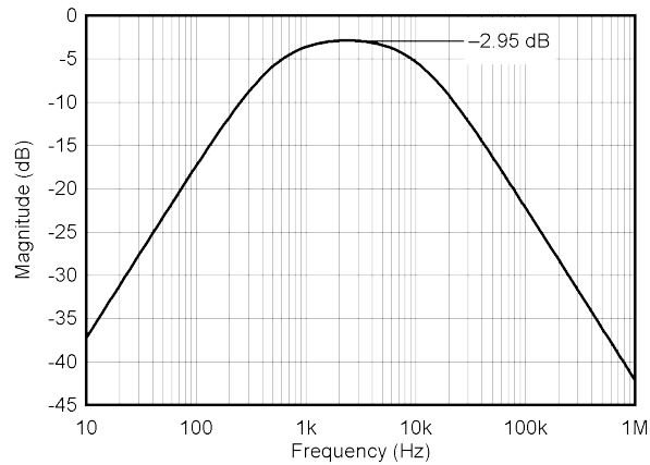
Figure 6-51. HART Internal Mode First Stage Band-Pass Filter Response (From HART_RX Signal to RX_INF Pin)
