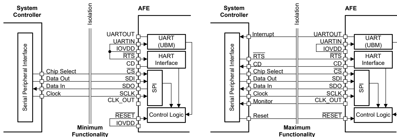
Figure 7-26. SPI Mode Connections
