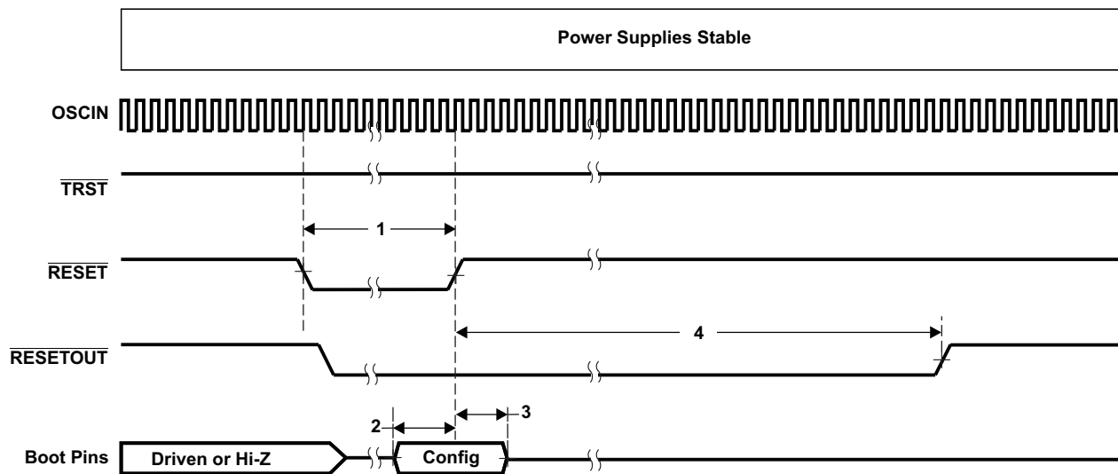
Figure 6-5. Warm Reset ( \overline{RESET} active, \overline{TRST} high) Timing
