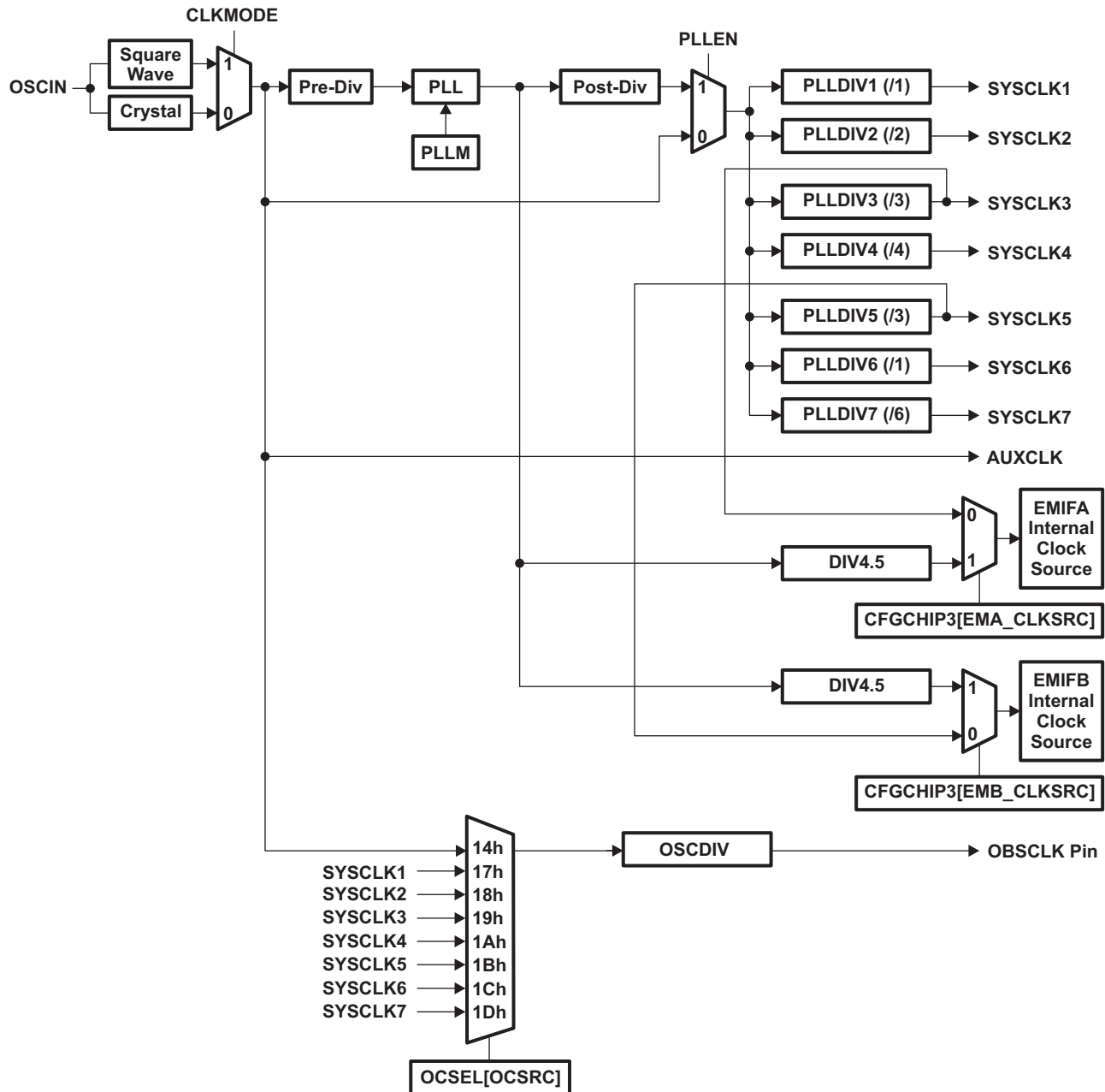
Figure 6-9. PLL Topology
