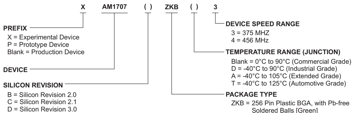
Figure 7-1. Device Nomenclature
