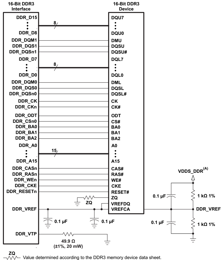
Figure 7-48. 16-Bit DDR3 Interface Using One 16-Bit DDR3 Device without V_{\Pi} Termination
