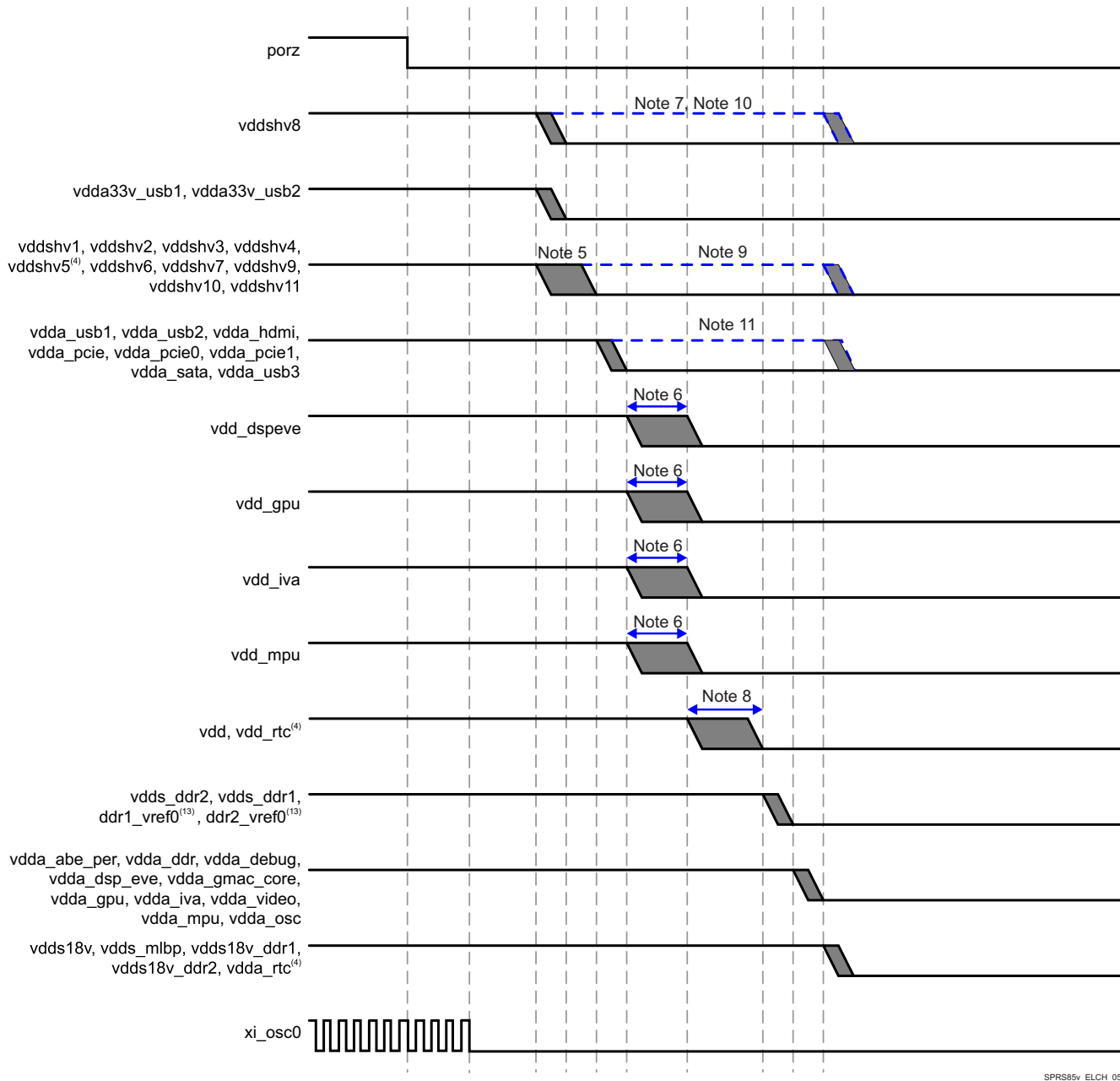
Figure 5-6. Power-Down Sequencing (12)(14)
