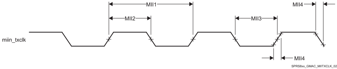
Figure 5-69. Clock Timing (GMAC Transmit) - MII n operation
