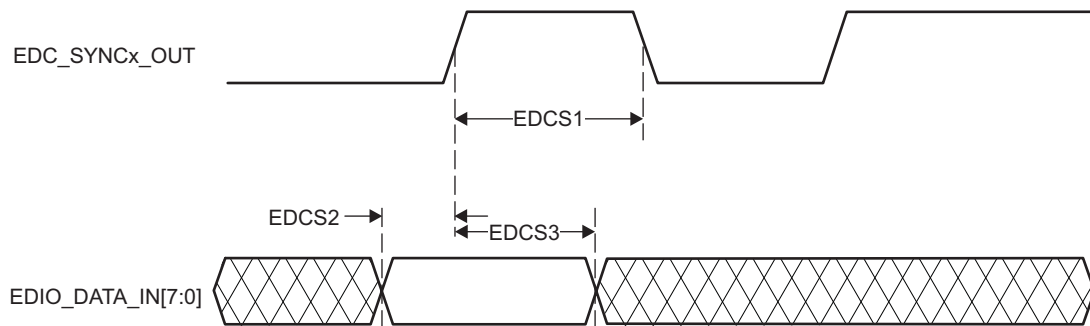
SPRS91x_TIMING_PRU_ECATCH_02
