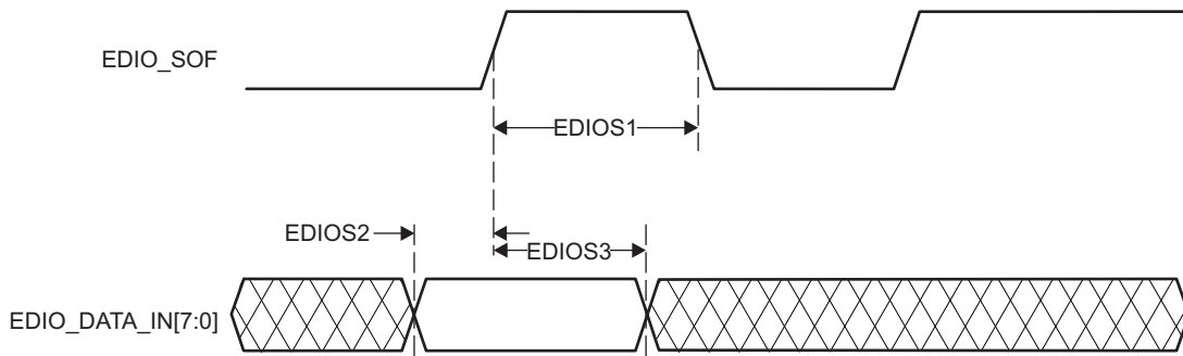
SPRS91x_TIMING_PRU_ECAC_03
