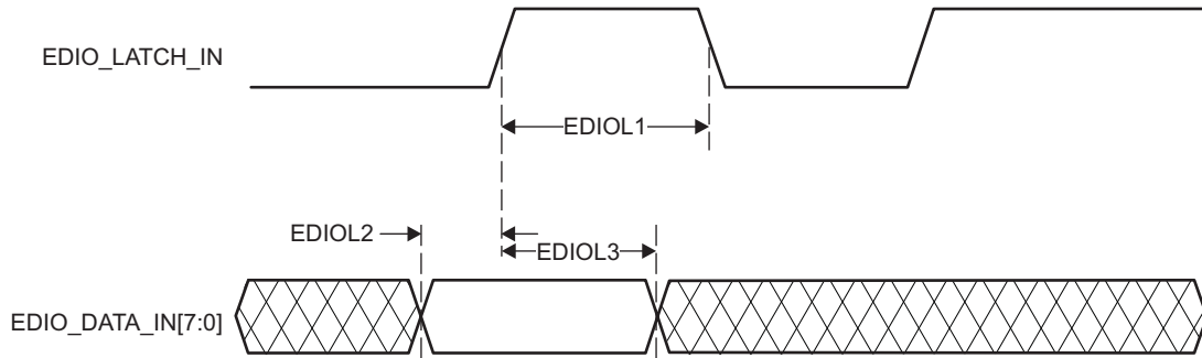
SPRS91x_TIMING_PRU_ECATCH_01
