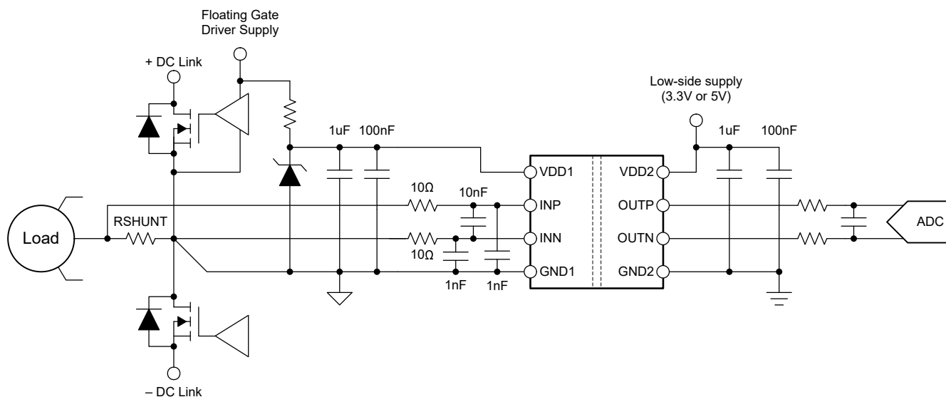
Figure 8-1. Using the AMC0x02D for Current Sensing in a Typical Application
