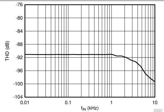
Figure 27. Total Harmonic Distortion vs Input Signal Frequency
