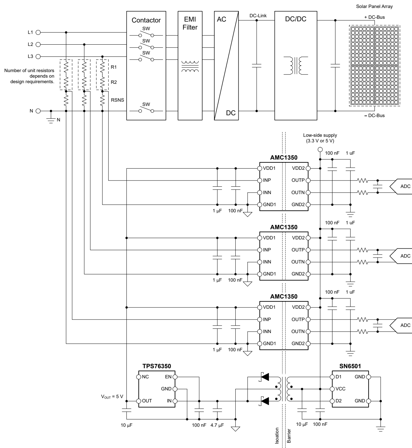
Figure 8-1. Using the AMC1350 for AC Line-Voltage Sensing in a Solar Inverter Application
