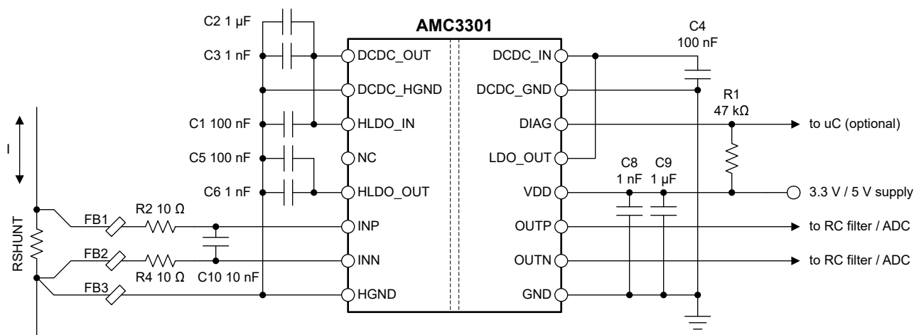
Figure 7-5. Decoupling the AMC3301
