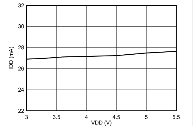
Figure 6-39. Supply Current vs Supply Voltage
