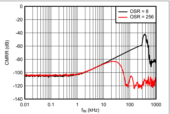
Figure 6-37. Common-Mode Rejection Ratio vs Input Signal Frequency
