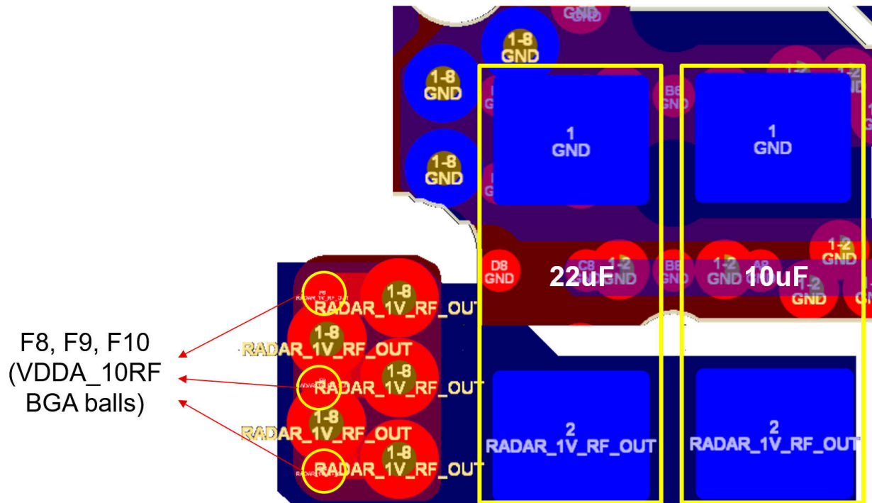
Figure 7-6. EVM Layout Example
