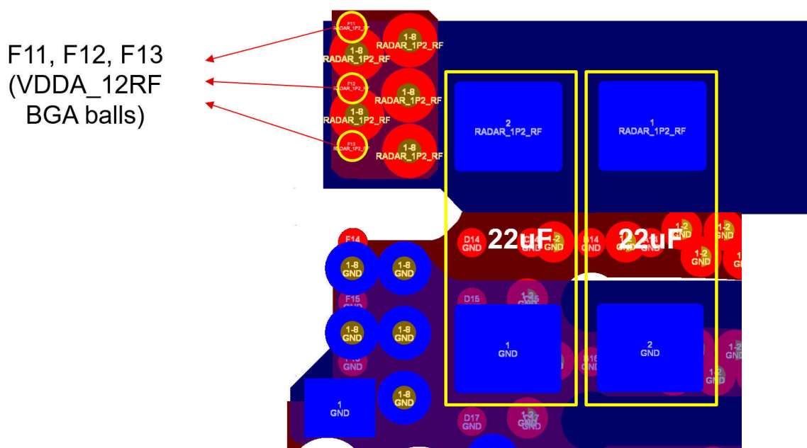
Figure 7-4. EVM Layout example
