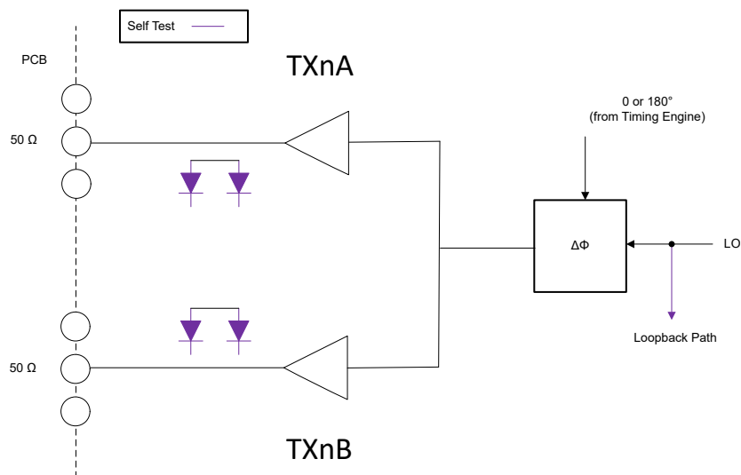
Figure 8-3. Transmit Subsystem (Per Two Transmit Channel Pair)
