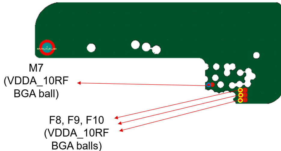
Figure 7-7. EVM Layout Example
