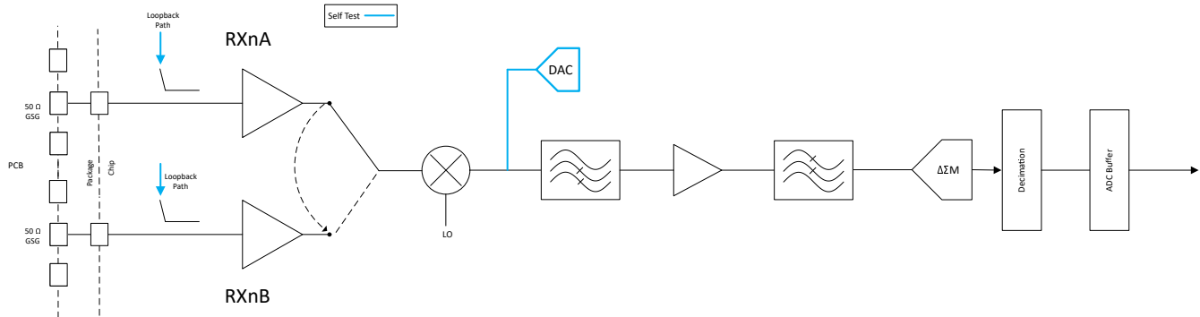
Figure 8-4. Receive Subsystem (Per Receive Channel Pair)
