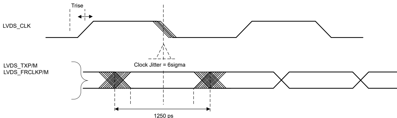
Figure 7-18. Timing Parameters
