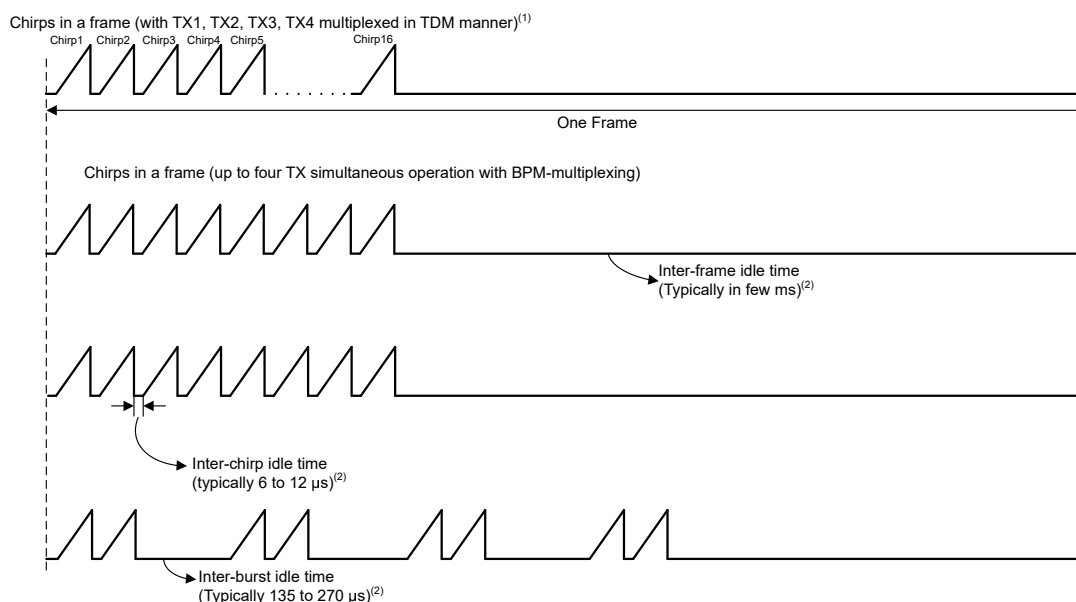
Figure 7-9. Chip Profile Supported by Timing Engine
