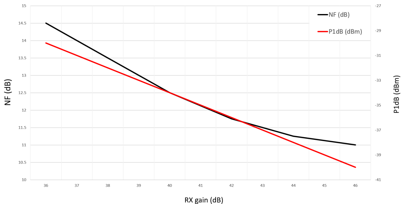
Figure 7-8. Noise Figure, In-band P1dB vs Receiver Gain
