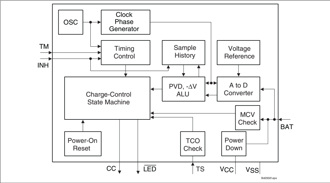
Figure 3. Block Diagram
