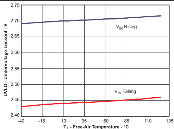
Figure 2. UVLO vs Free-Air Temperature
