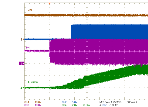
CH1: Vin, 10 V/div, CH2: LODRV, 5 V/div, CH3: PHASE, 10 V/div, CH4: inductor current, 2 A/div, 2 ms/div
