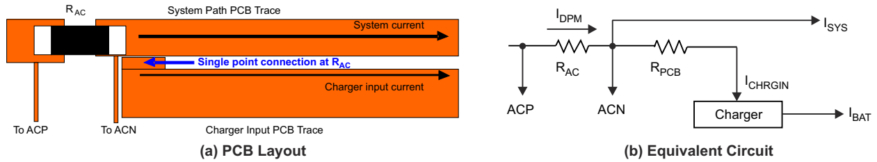
Figure 7-27. Optimized PCB Layout Example
