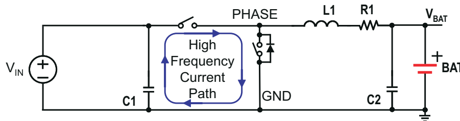
Figure 7-23. High Frequency Current Path
