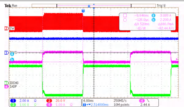
Figure 7-17. Hybrid Power Boost Mode With Discharge Current Regulation
