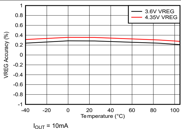
Figure 5-5. VSET Accuracy vs Temperature
