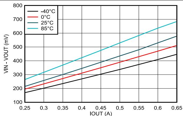
Figure 5-6. Dropout Voltage vs Output Current
