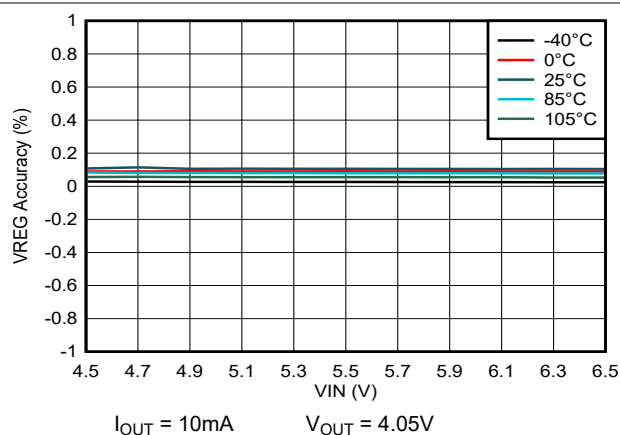
Figure 5-1. Line Regulation
