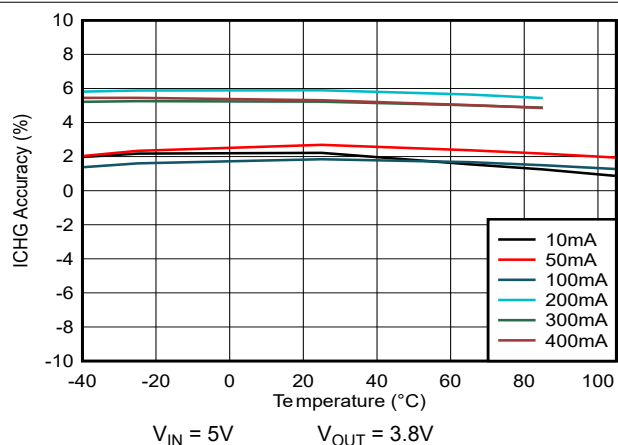
Figure 5-4. ICHG Accuracy vs Temperature
