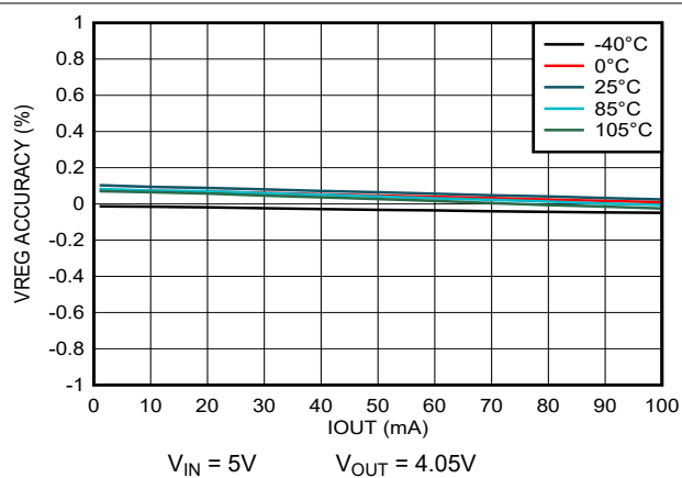
Figure 5-2. Load Regulation
