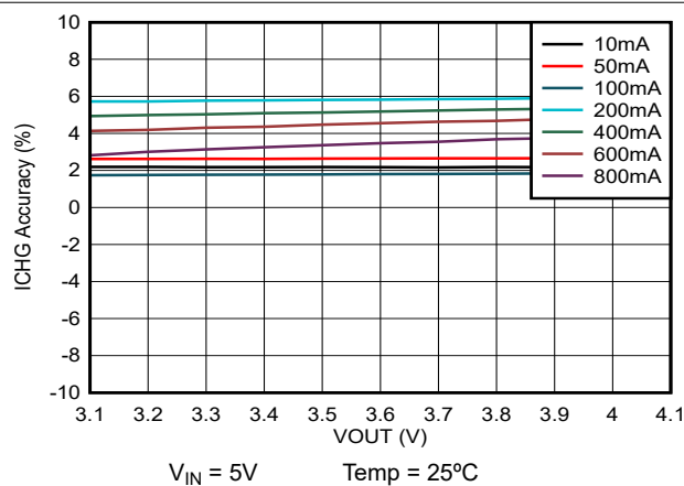
Figure 5-3. ICHG Accuracy vs V_{OUT}
