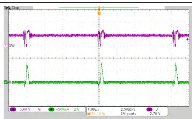
Figure 10-9. Charge Enable
