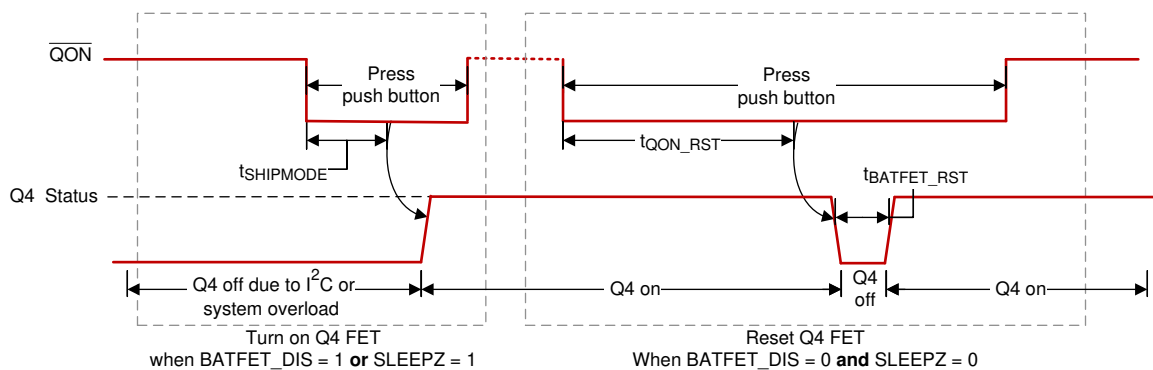
Figure 9-10. \overline{\text{QON}} Timing
