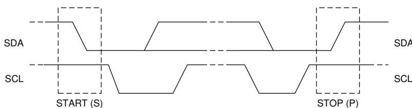
Figure 9-13. TS START and STOP Conditions
