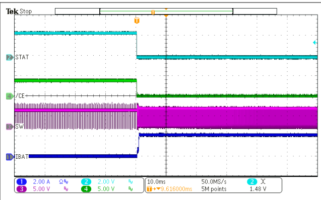
Figure 10-9. Charge Enable
