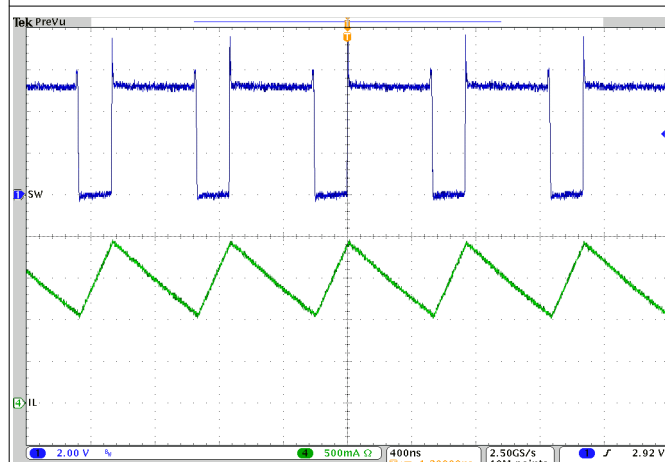
Figure 10-10. Charge Disable
