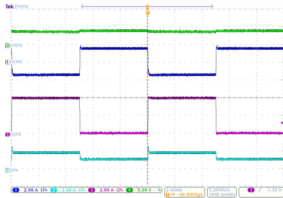
Figure 8-8. System Load Transient Response
