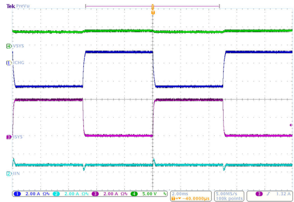
Figure 8-7. System Load Transient Response
