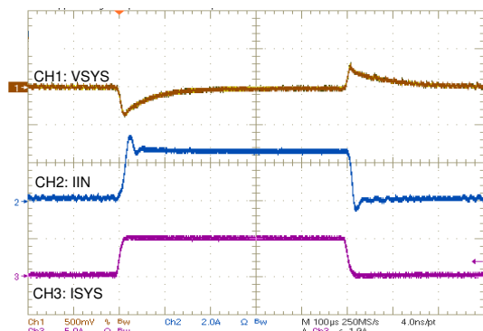
Figure 10-9. Switching During Boost Mode
