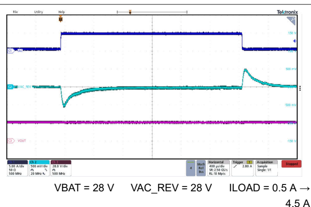
Figure 9-16. Reverse Mode Buck-Boost Transient Reponse
