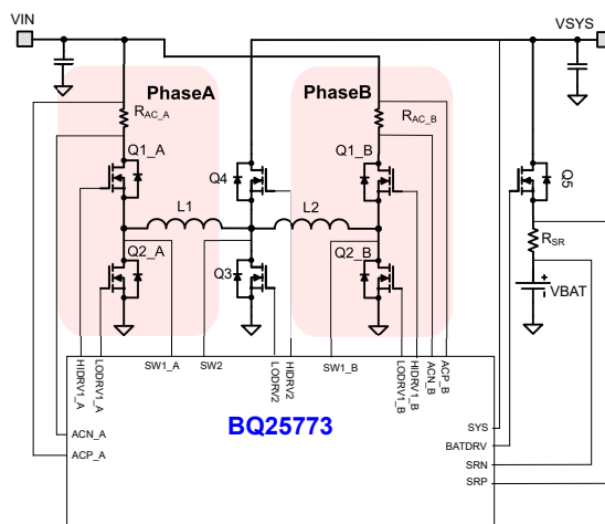
Application Diagram
