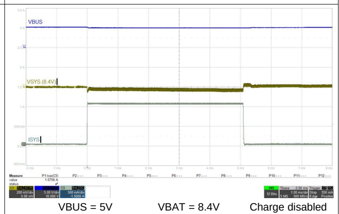
Figure 84. System Load Transient Response
