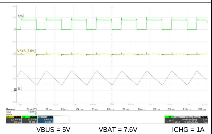
Figure 82. Boost Mode PWM Switching
