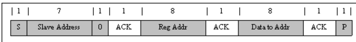
Figure 29. Single Write
